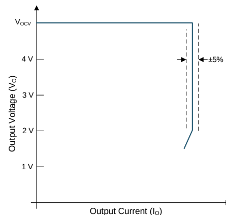
Typical V-I Diagram
