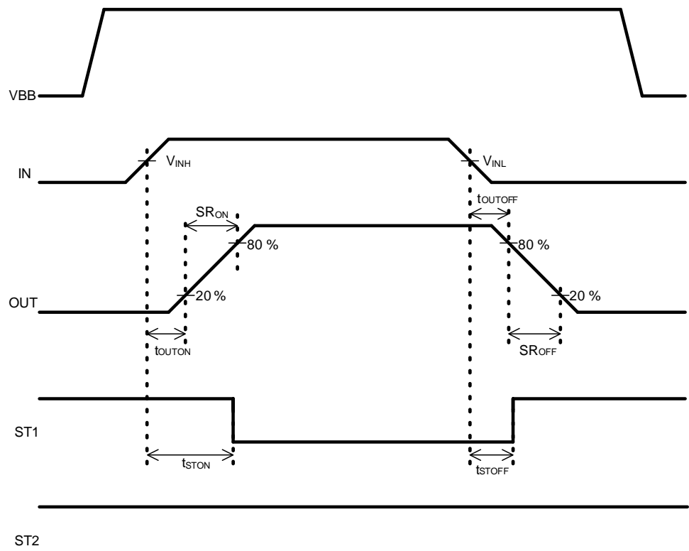
Figure 34. Timing Chart
