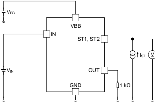
Figure 30. Diagnostic Output Low Voltage
