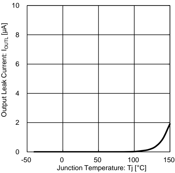
Figure 16. Output leak Current vs Junction Temperature
