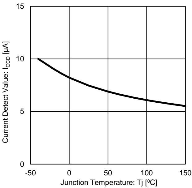
Figure 23. Current Detect Value vs Junction Temperature
