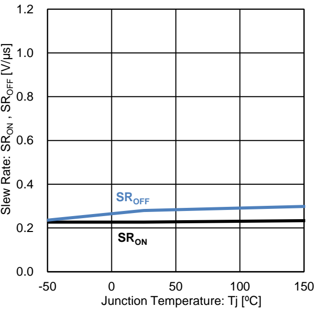
Figure 17. Output Slew Rate vs Junction Temperature
