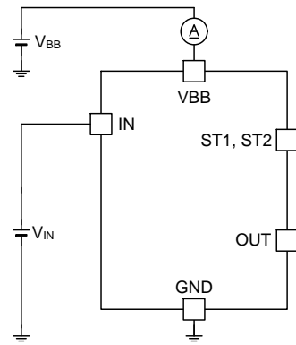
Figure 26. Operating Current
