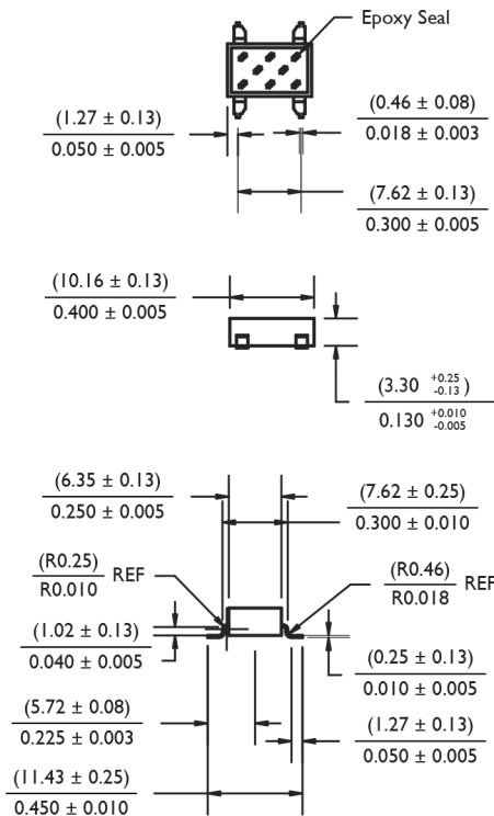
Surface Mount (Gullwing, SMT) Configuration
