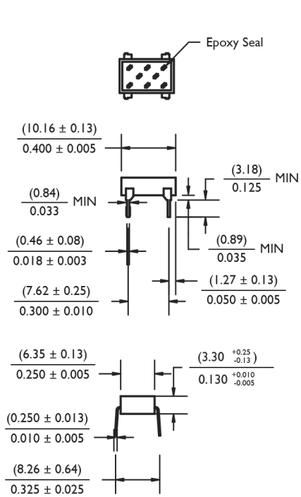
Standard 8-Pin DIP Configuration
