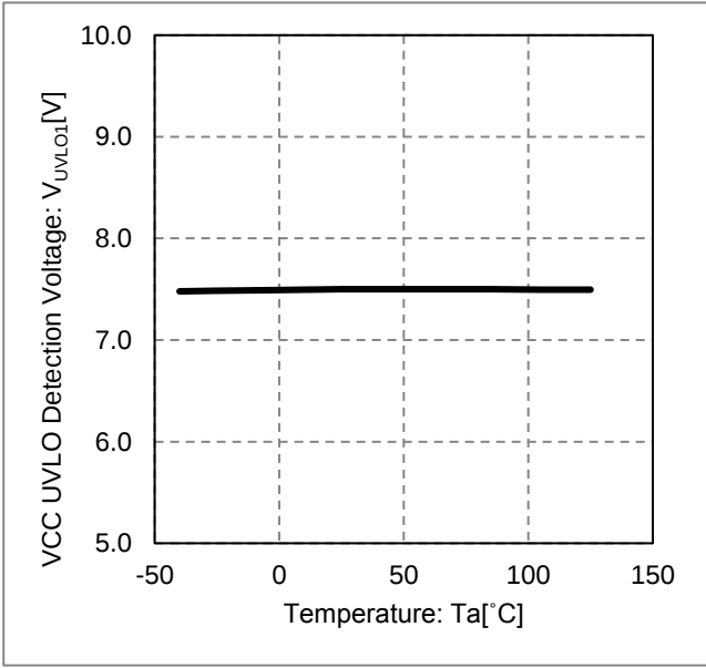
Figure 23. VCC UVLO Detection Voltage vs Temperature
