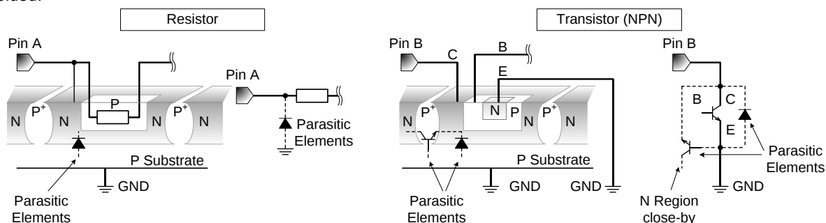
Figure 33. Example of IC Structure
