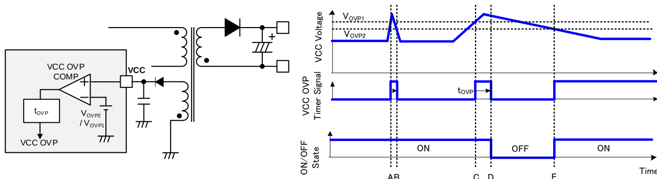
Figure 11. VCC OVP Block Diagram and Timing Chart
