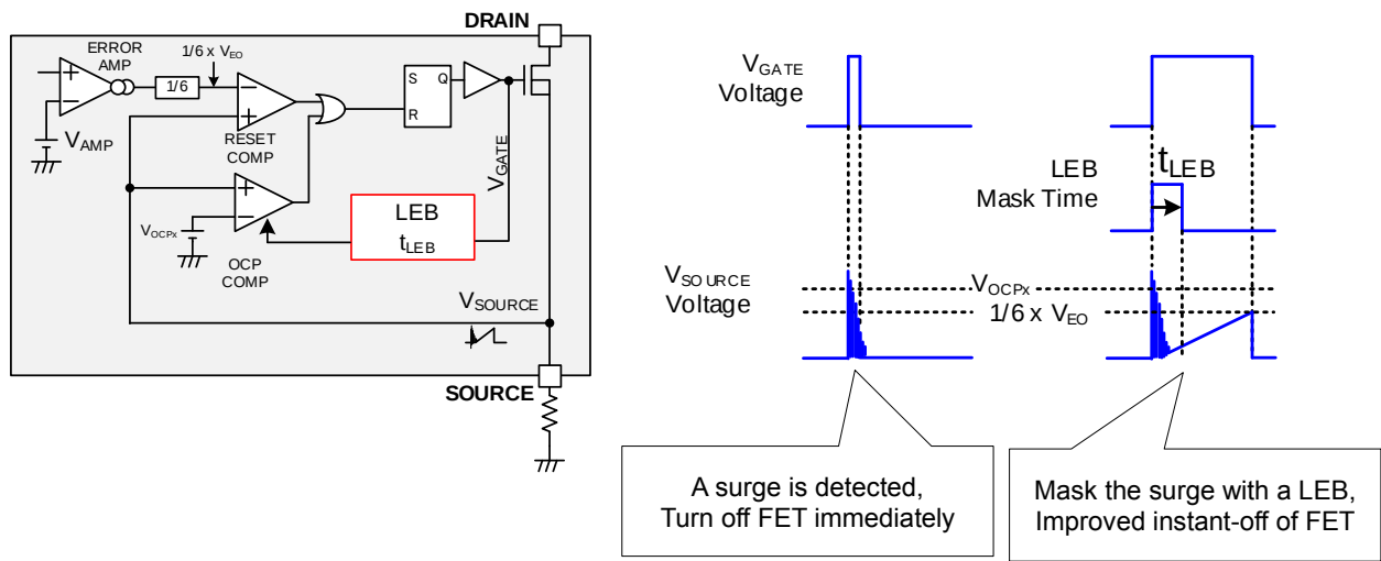
Figure 9. LEB Block Diagram and Timing Chart
