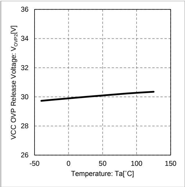
Figure 28. VCC OVP Release Voltage vs Temperature
