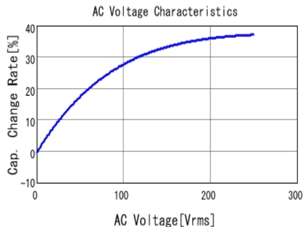
■ DE1E3KX102MA4BN01F C-AC Voltage capchange, DC0V, 20.0
