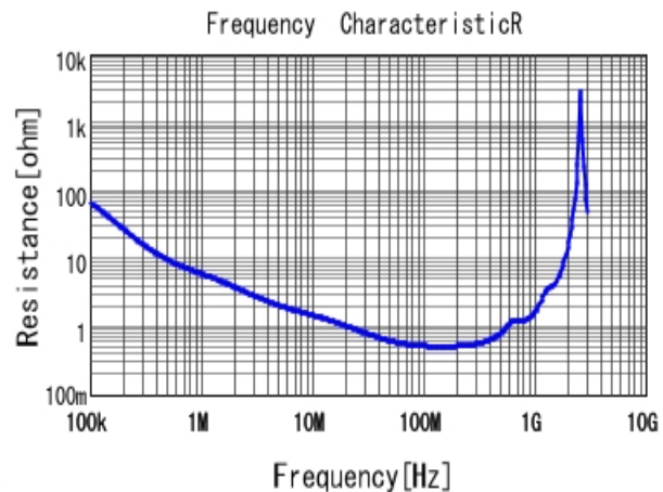
■ DE1E3KX102MA4BN01F R DC0V, 20degC
