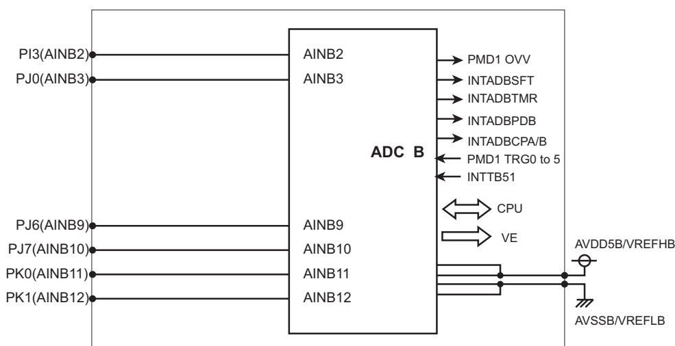
Figure 11-1 AD converters Block Diagram
