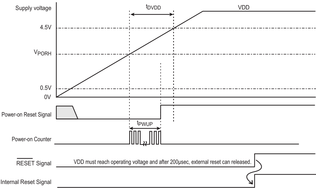
Figure 23-8 Power on Sequence ( t_{DVDD} > t_{PWUP} )
