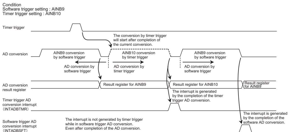
Figure 11-8 AD conversion by timer trigger (1)
