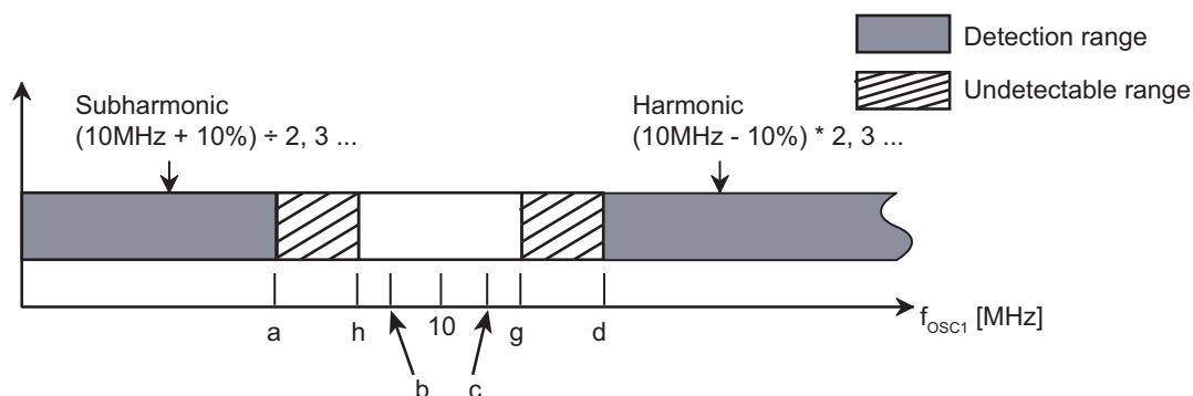
Figure 17-3 Example of detection frequency range (in case of 10MHz)
