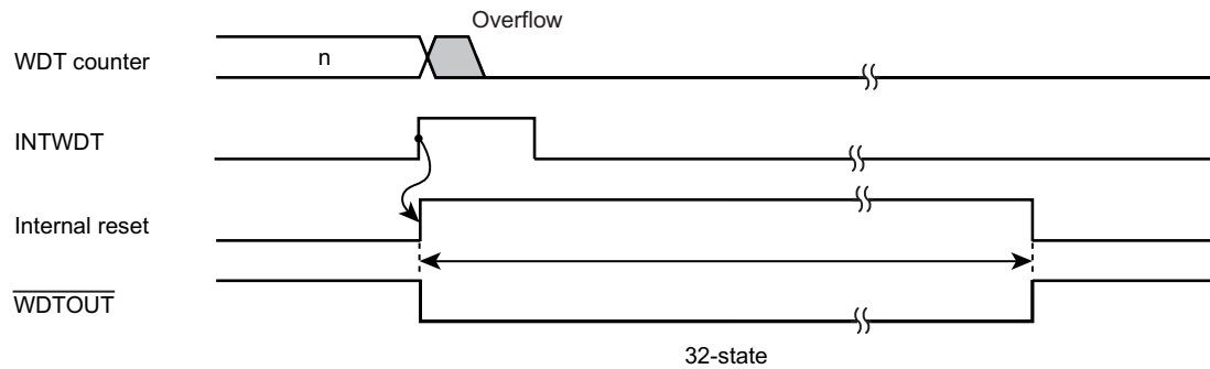
Figure 18-3 Internal reset generation
