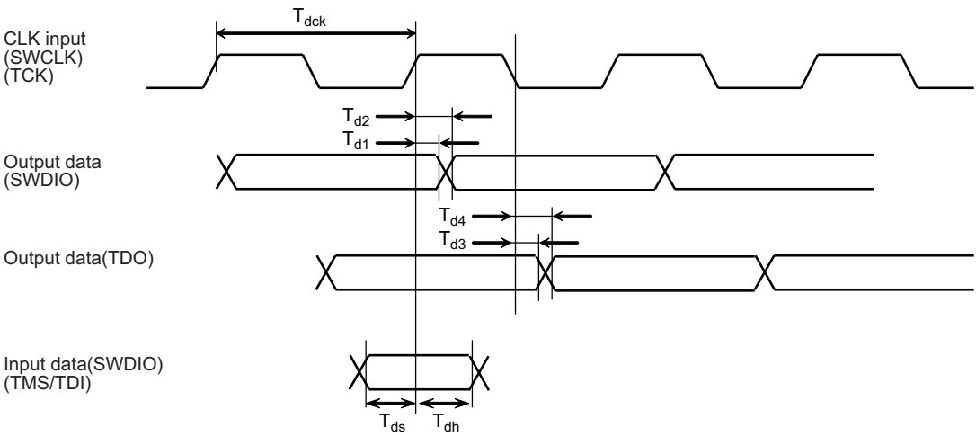
Figure 23-2 JTAG and SWD communication timing
