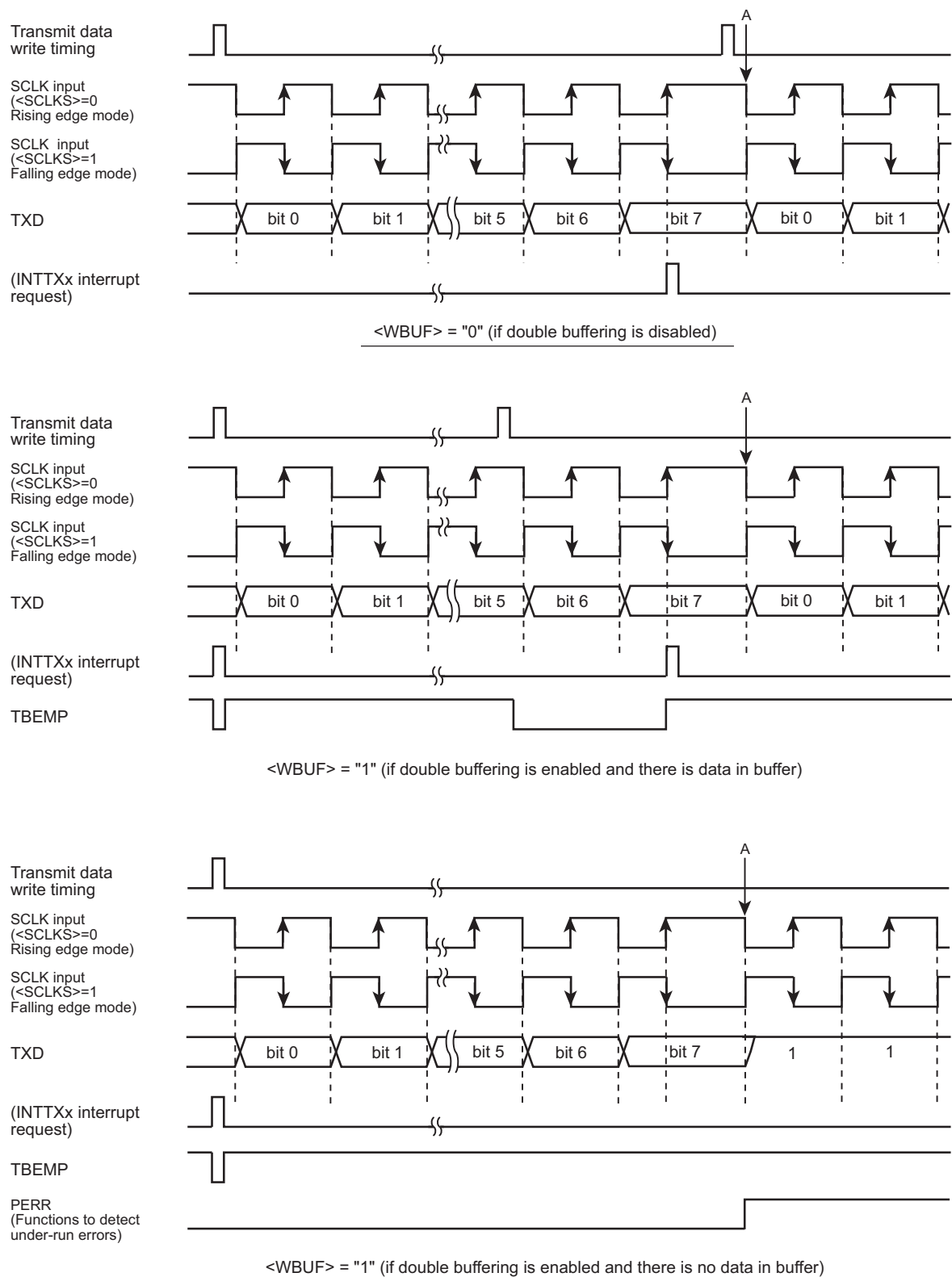
Figure 10-13 Transmit Operation in the I/O Interface Mode (SCLK Input Mode)
