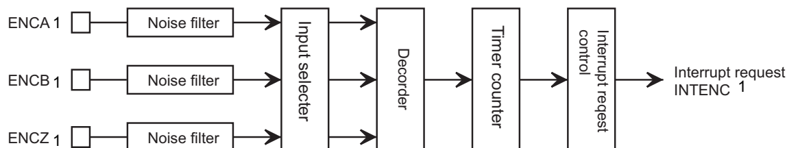
Figure 14-1 Block diagram of encoder input circuit
