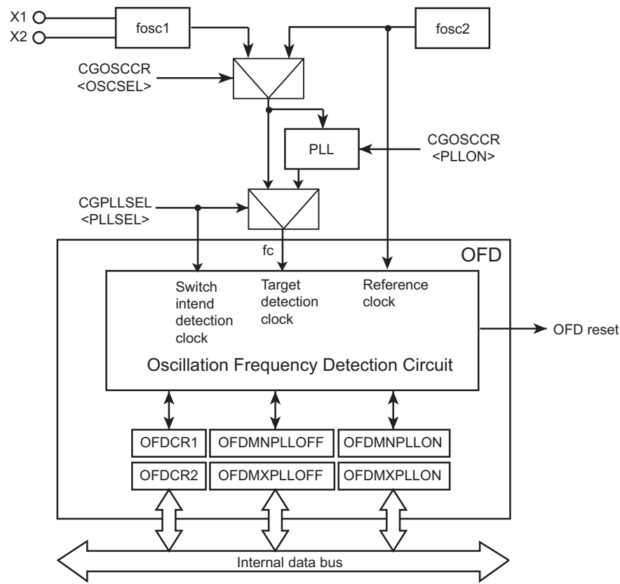
Figure 17-1 Oscillation Frequency Detector Block diagram
