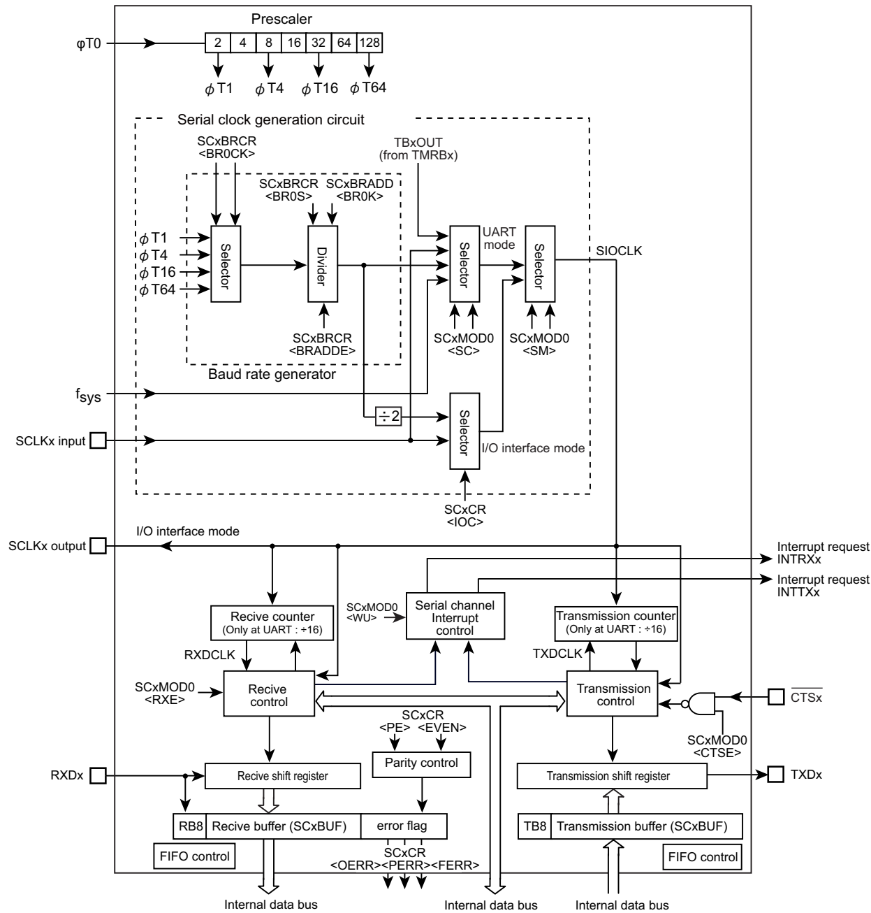
Figure 10-1 SIO Block Diagram
