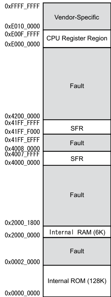
Figure 3-1 Memory Map
