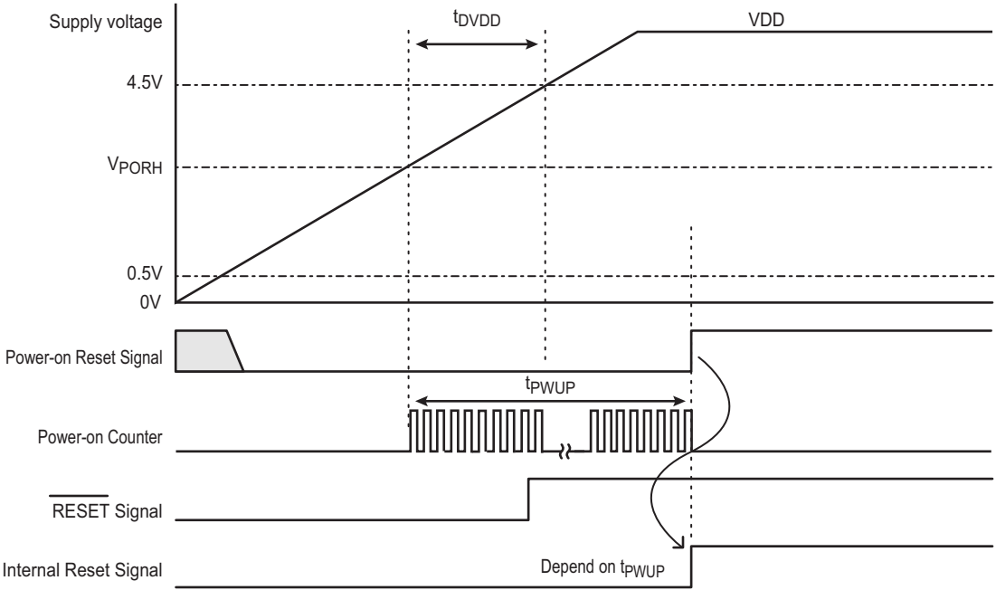
Figure 23-6 Power on Sequence ( Using POR and External reset ) (1)
