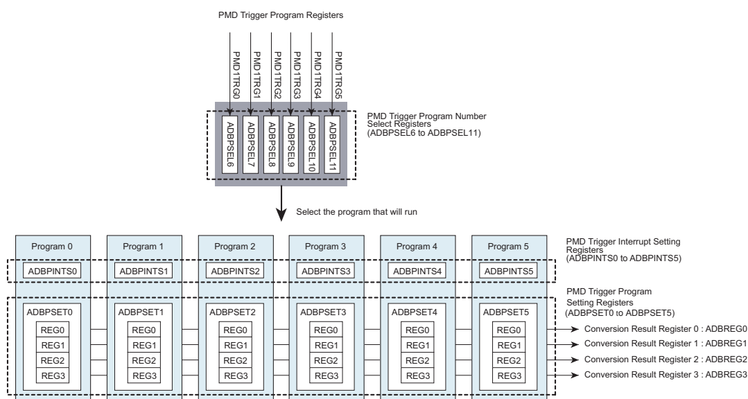
Figure 11-2 PMD Trigger Program Registers
