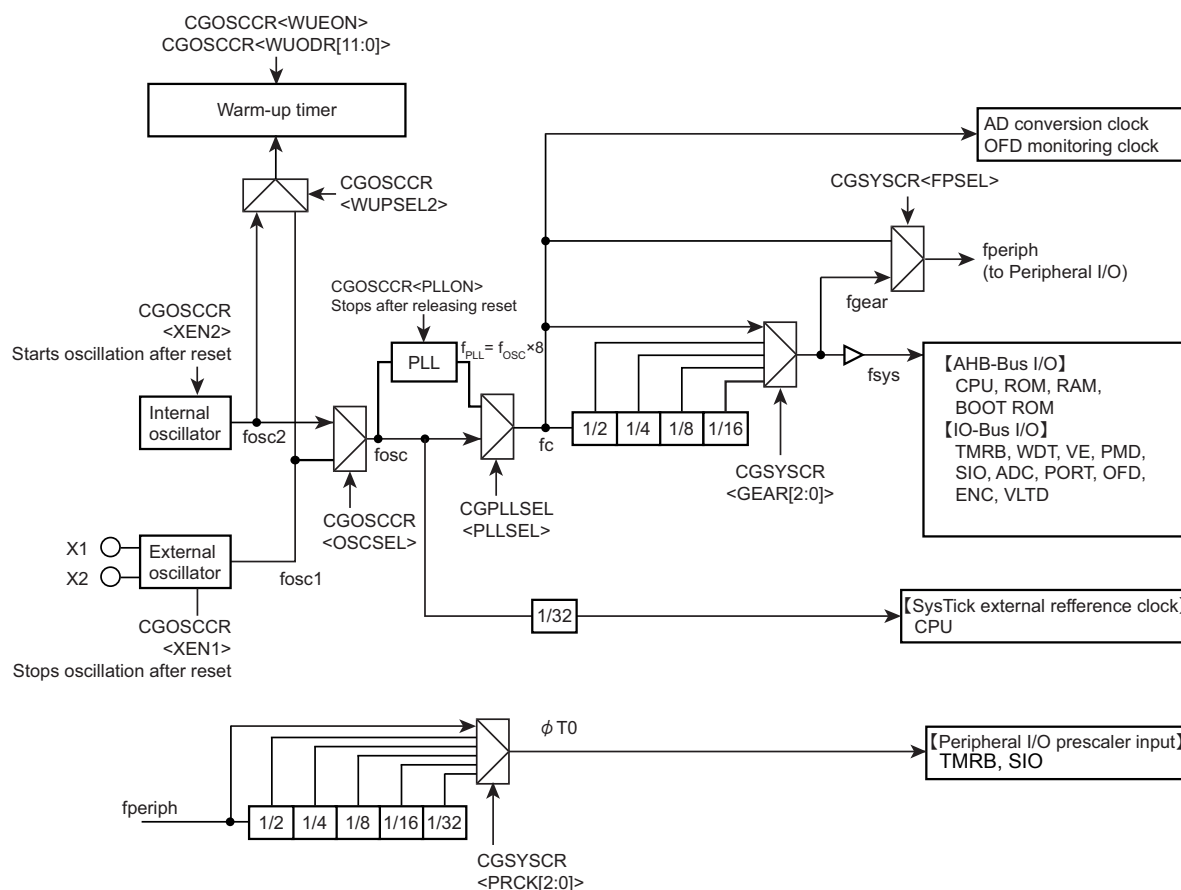
Figure 5-1 Clock Block Diagram
