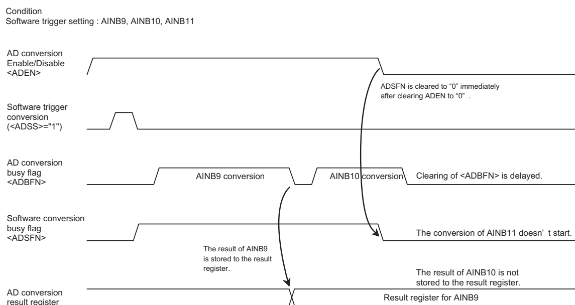
Figure 11-5 Writing "0" to <ADEN> during the software trigger AD conversion
