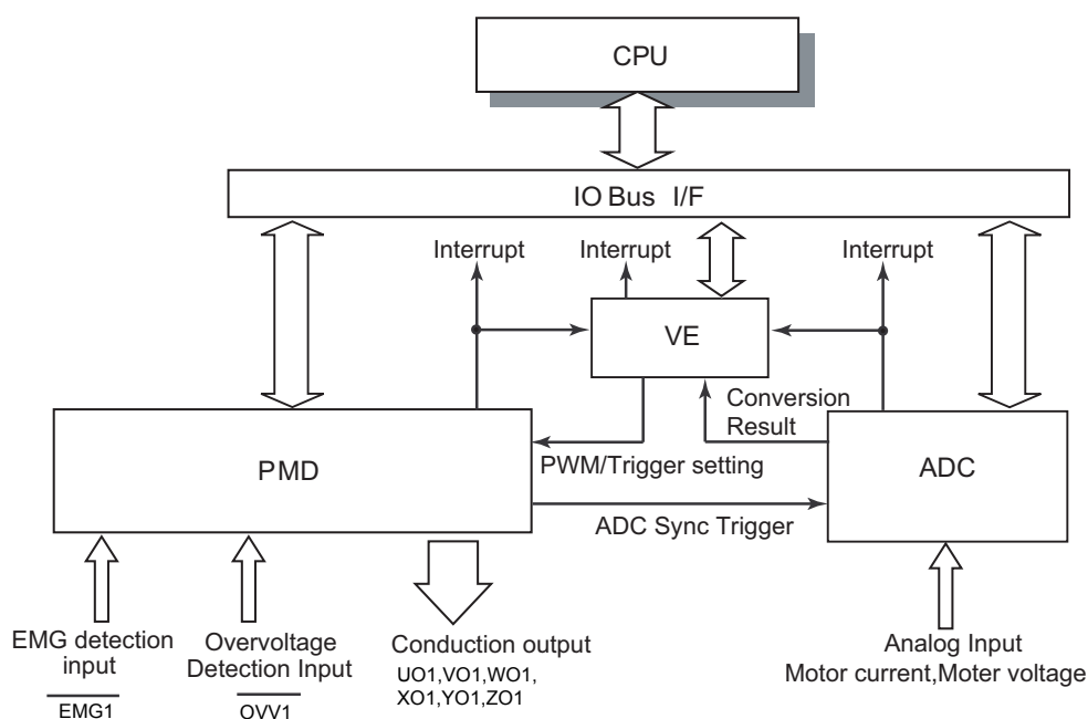
Figure 12-1 Motor Control-related Block Constitution
