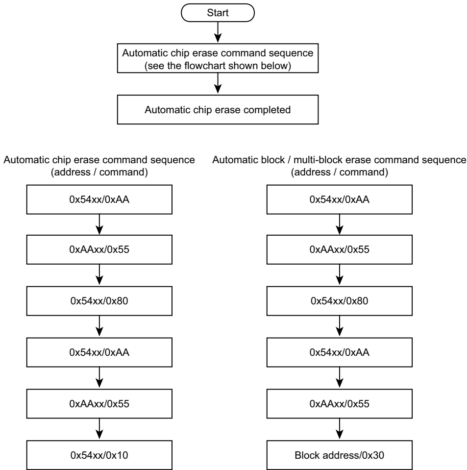
Figure 19-11 Automatic Erase
