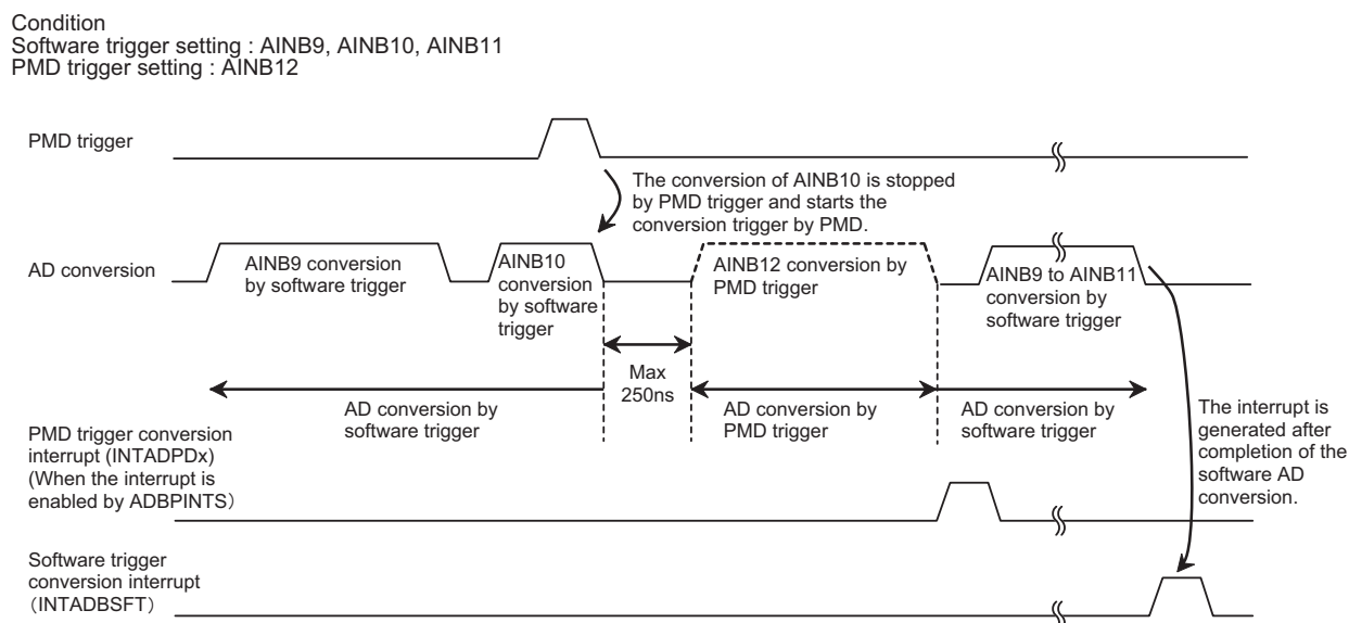
Figure 11-7 AD conversion by PMD trigger
