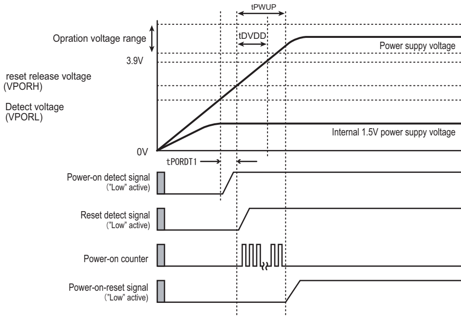
Figure 15-2 Power-on-reset operation timing
