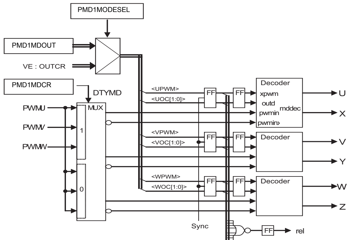
Figure 12-5 Conduction Control Circuit
