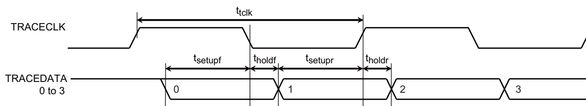
Figure 23-3 TRACE communication timing
