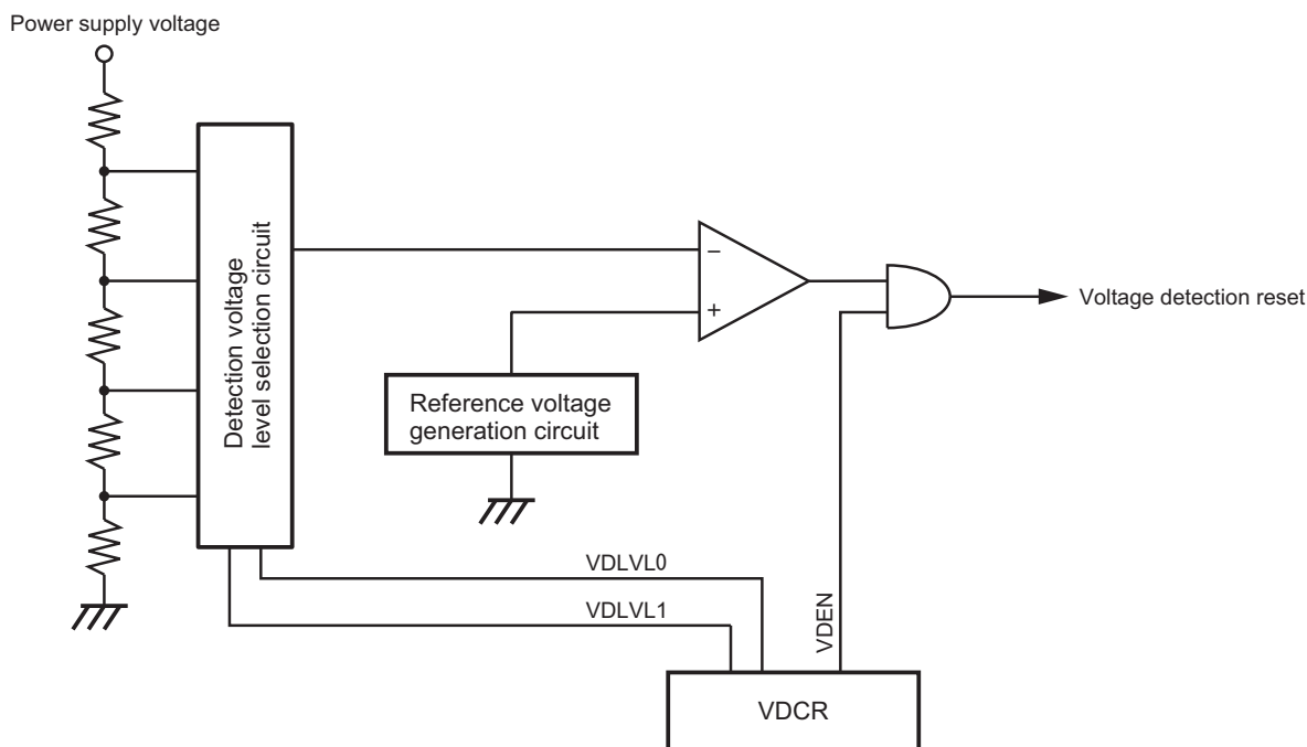
Figure 16-1 Voltage Detection Circuit)
