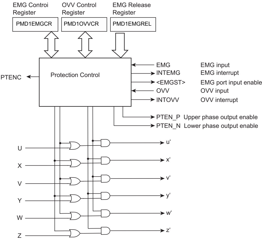
Figure 12-6 Protection Control Circuit
