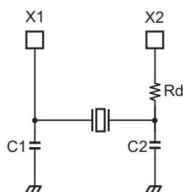
Figure 23-4 High-frequency oscillation connection
