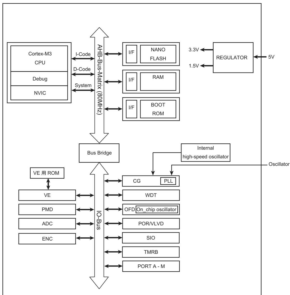
Figure 1-1 TMPM374FWUG block diagram
