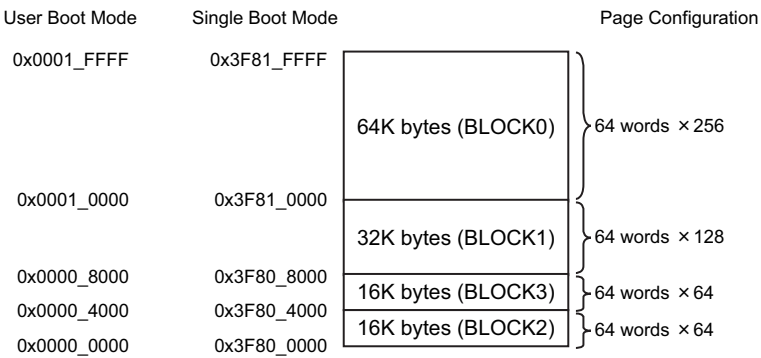
Figure 19-9 Block Configuration of Flash Memory (TMPM374FWUG)
