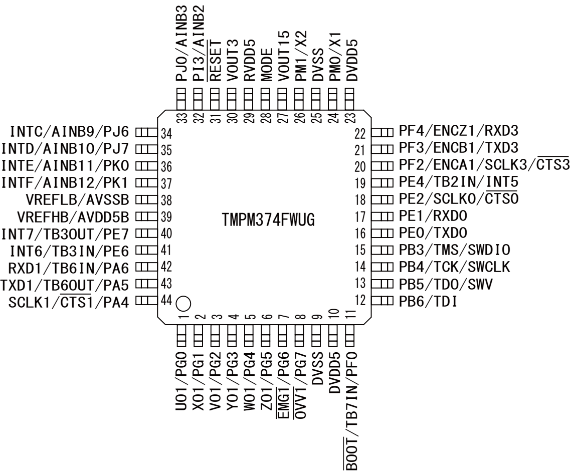
Figure 1-2 Pin Layout (LQFP44)
