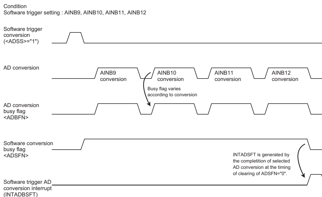
Figure 11-4 Software trigger AD conversion
