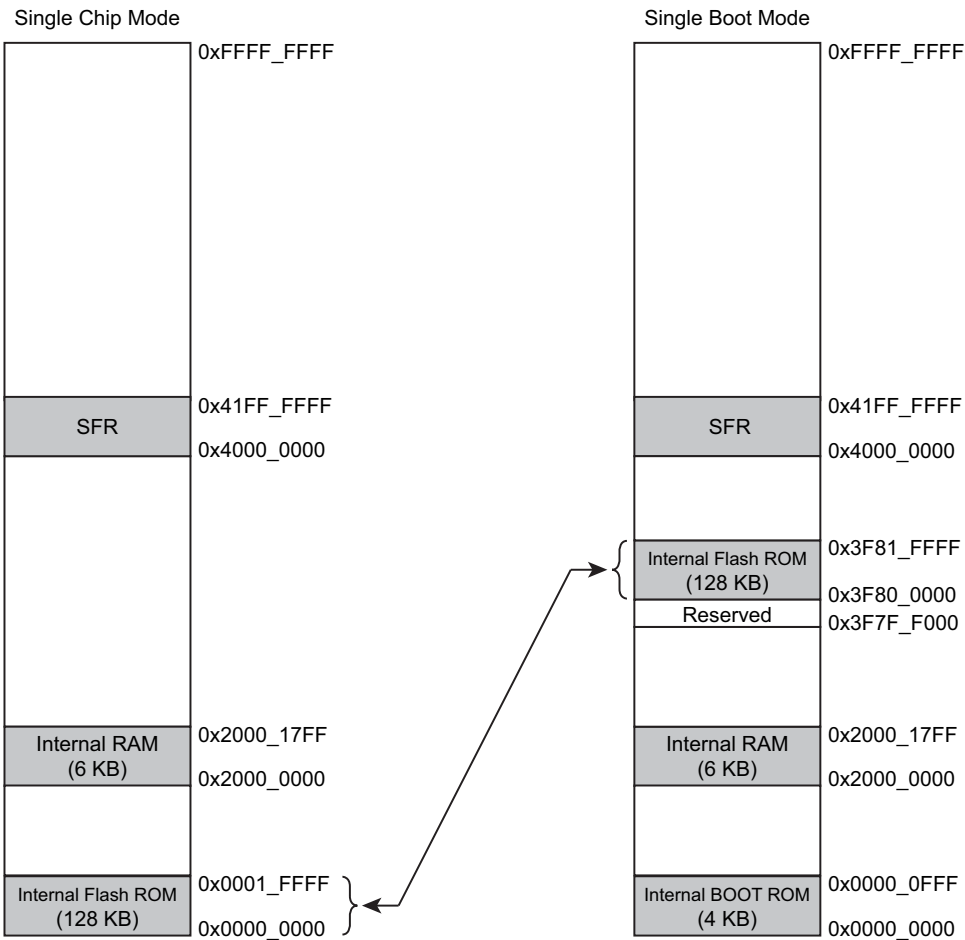
Figure 19-3 Memory Maps for TMPM374FWUG
