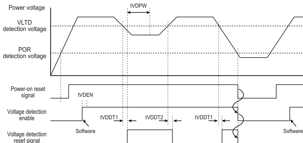
Figure 16-2 Voltage Detection Timing
