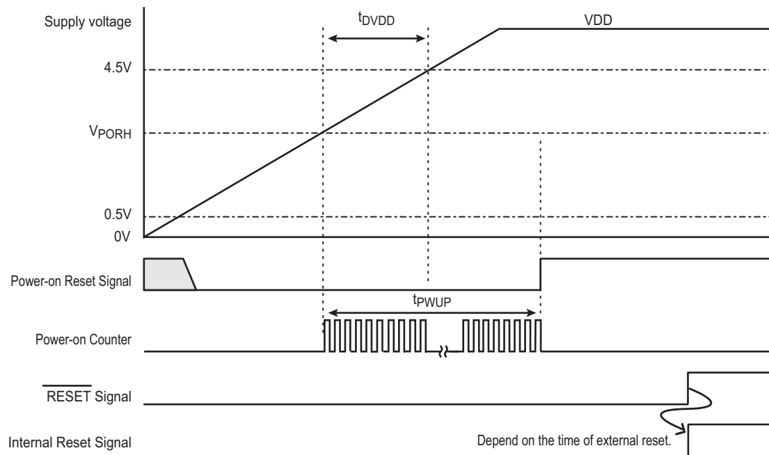
Figure 23-7 Power on Sequence ( Using POR and External reset ) (2)
