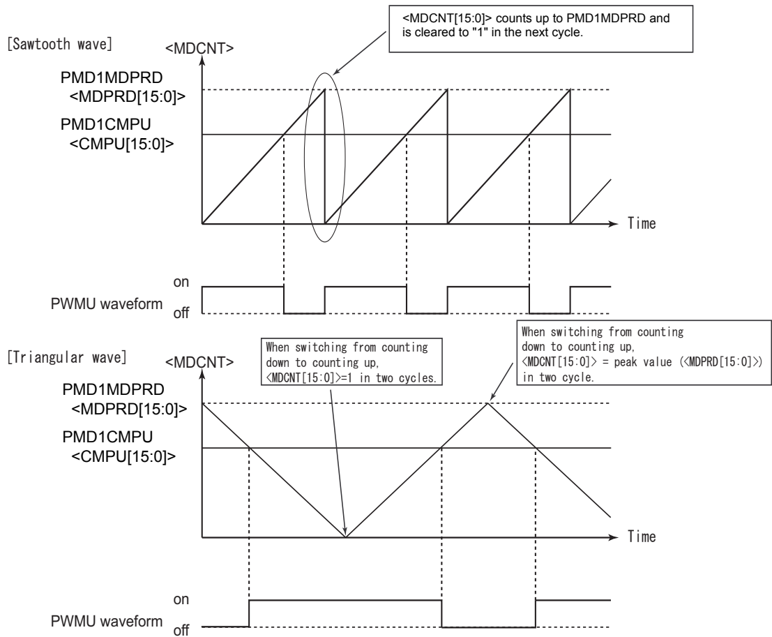
Figure 12-4 PWM Waveforms
