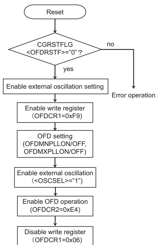
Figure 17-4 Example of operational procedure
