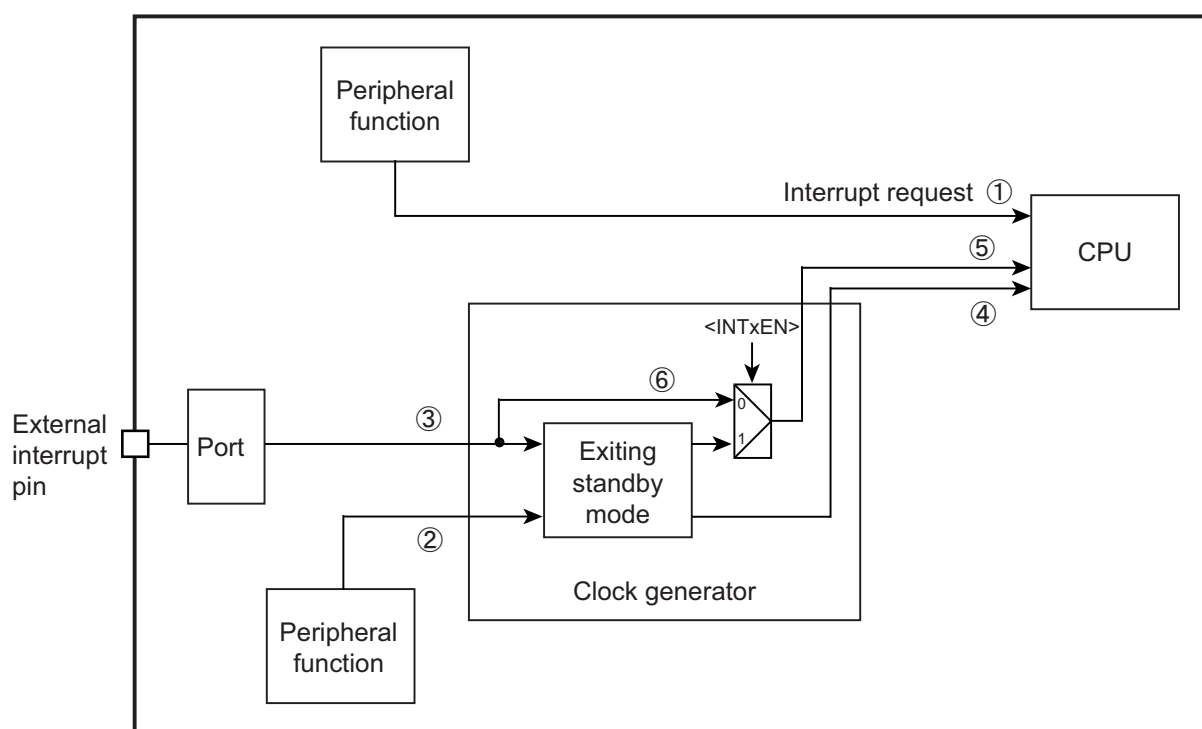
Figure 6-1 Interrupt Route
