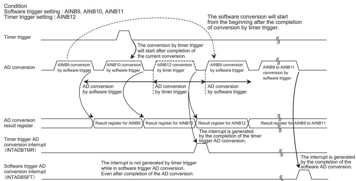
Figure 11-9 AD conversion by timer trigger (2)
