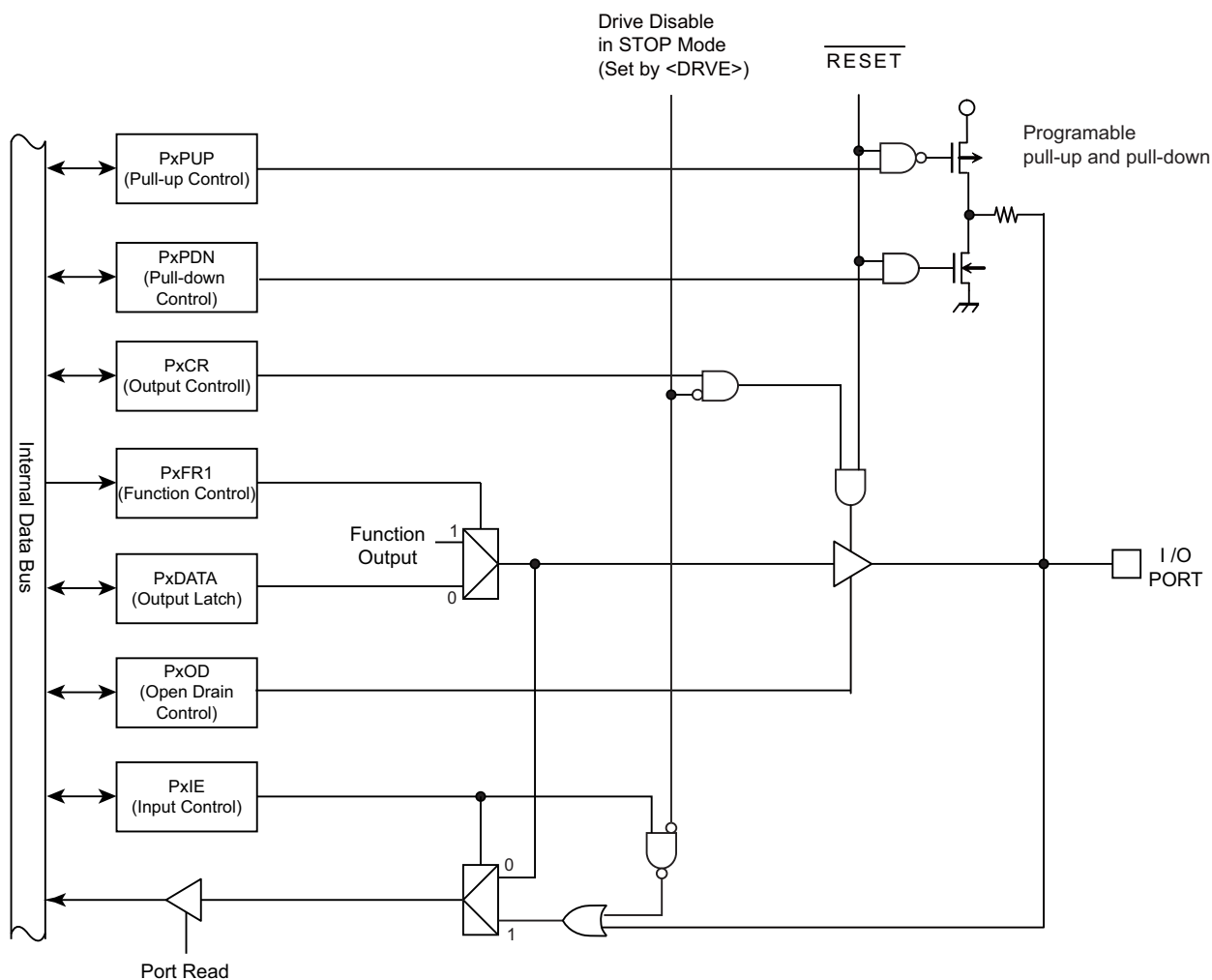
Figure 8-2 PORT Type T2
