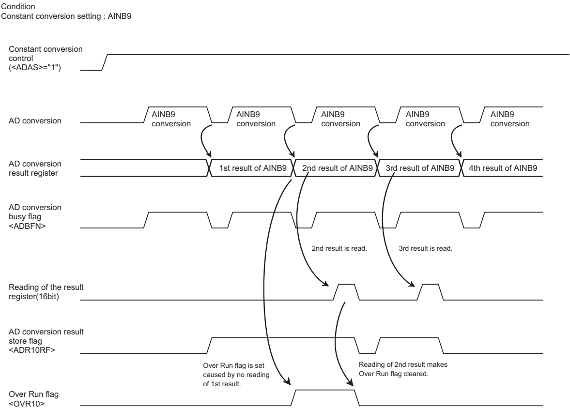
Figure 11-6 Constant conversion
