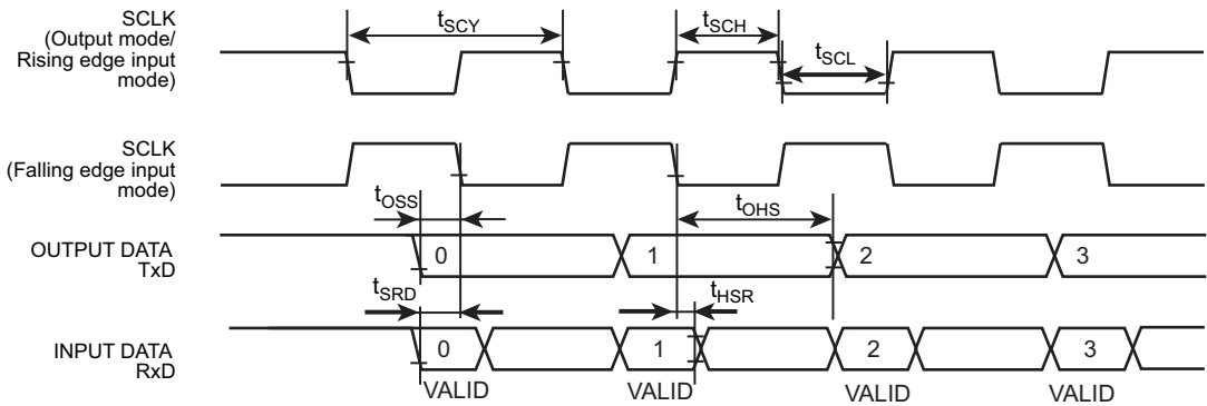
Figure 23-1 Serial channel timing(SIO/UART)
