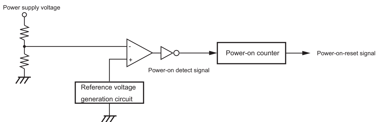
Figure 15-1 Power-on-reset circuit
