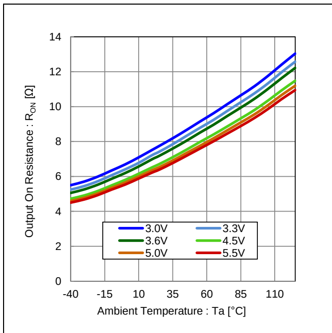
Figure 11. Output On Resistance vs Ambient Temperature (@I Dn =20mA)
