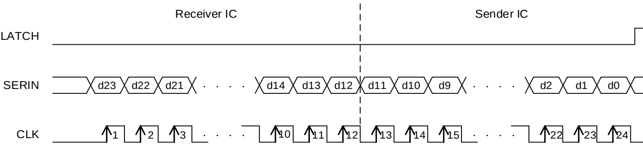
Figure 7. Cascade Connection
