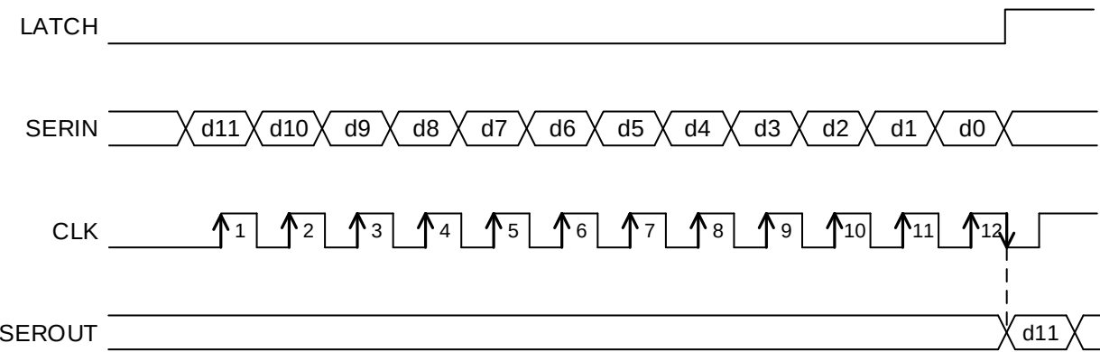
Figure 6. SEROUT Output Signal
