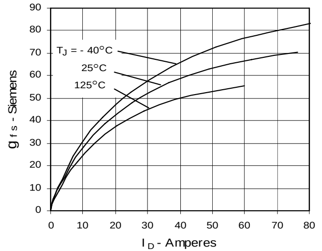
Fig. 8. Transconductance
