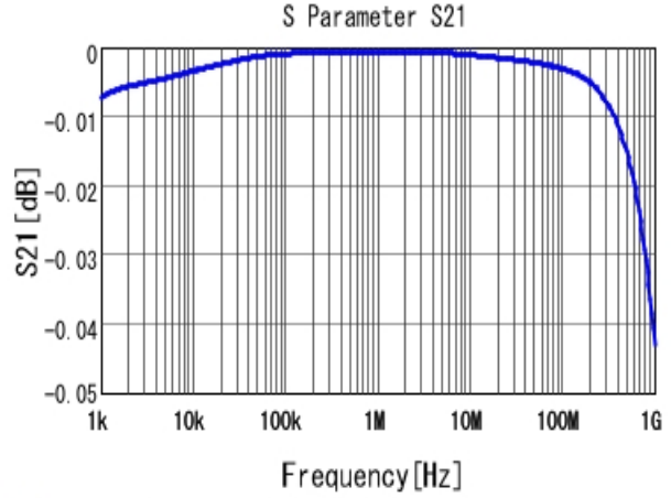
■ ECASD40J686M015K00 S21 DCOV, 25degC
