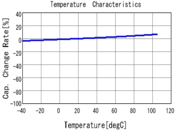
■ ECASD40J686M015K00 C-Temp. capchange, DCOV, AC1Vrms
