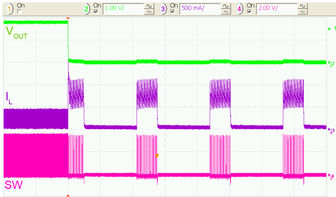
Figure 33. Metallic Short Applied at V_{OUT} , 50\text{ }\mu\text{s/div.}
