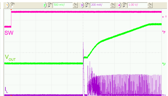
Figure 38. Soft-Start, R_{LOAD} = 50\text{ }\Omega , 20\text{ }\mu\text{s/div.}
