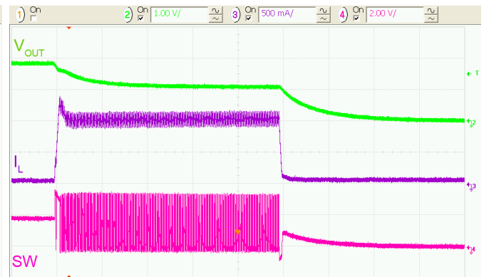
Figure 36. Over-Current Fault Response, R_{LOAD} = 1\text{ }\Omega
