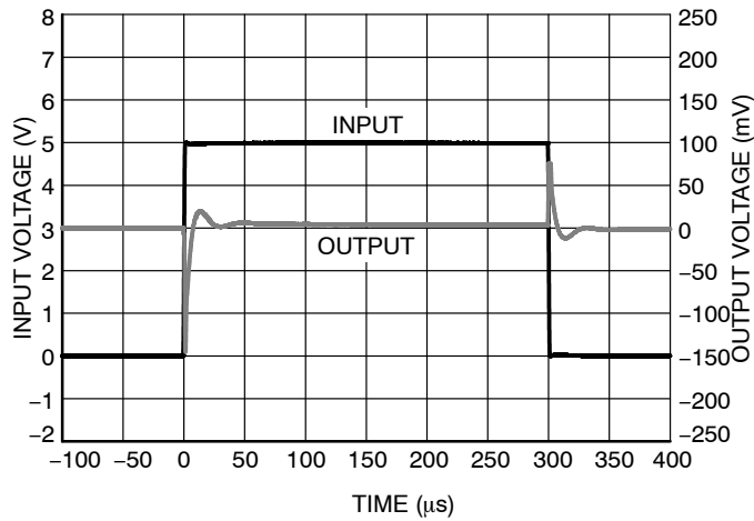
Figure 25. Common-Mode Voltage Transient Response
