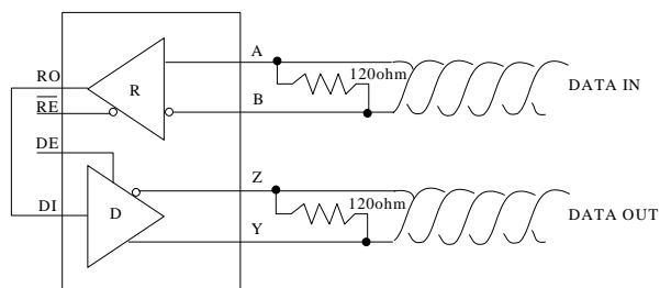
Figure 12: Line Repeater
