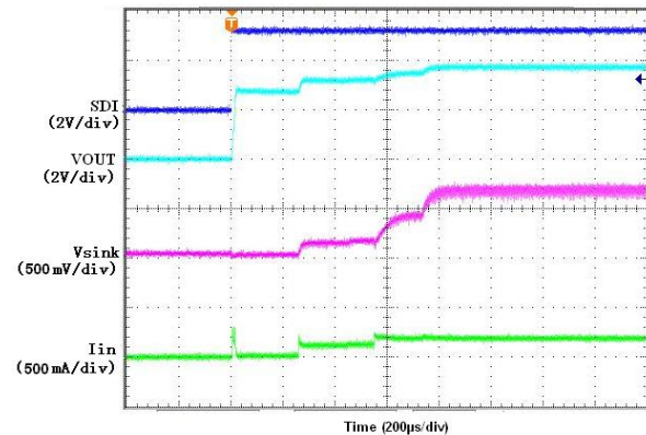
Turn-On to 2X Mode ( V_{IN} = 2.7V ; 20mA Load)
