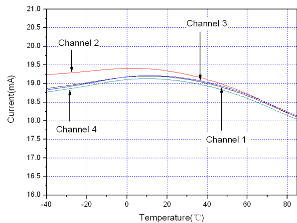
Current Matching vs. Temperature
