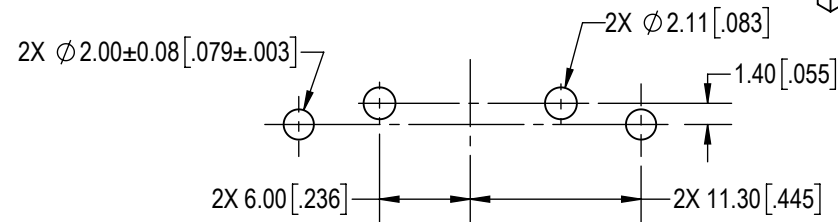
CONTACT HOLE PATTERN
