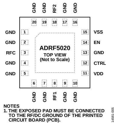
Figure 5. Pin Configuration (Top View)
