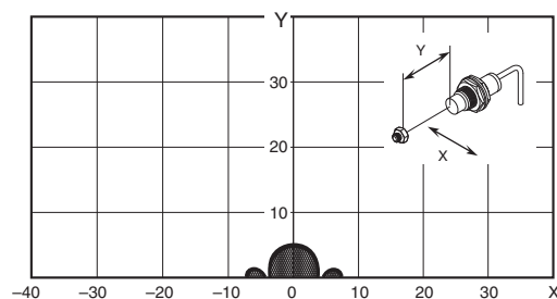
V680-D1KP52M-BT11 (mounted in metal/non-metallic material)
