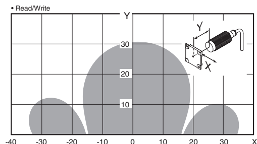
V680-HS65 (mounted in metal) & V680S-D8KF67M (mounted on metallic surface: steel)
