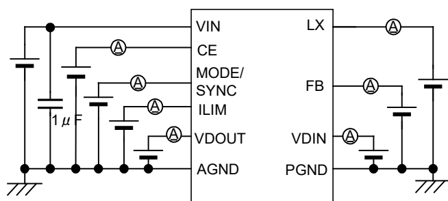
Circuit ⑥
