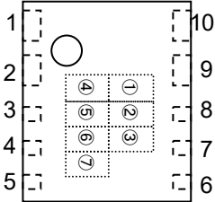
USP-10B (BOTTOM VIEW)
