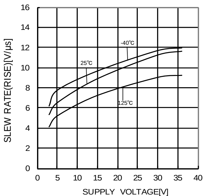
Figure 20. Slew Rate L-H - Supply Voltage ( R_L=10k\Omega )
