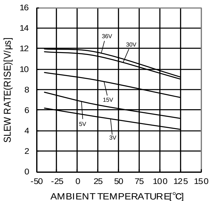
Figure 21. Slew Rate L-H Ambient Temperature ( R_L=10k\Omega )
