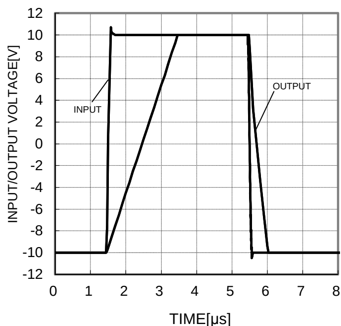
Figure 46. Input / Output Voltage - Time ( V_{CC}/V_{EE}=+15V/-15V , A_v=0dB , R_L=2k\Omega , C_L=100pF , T_a=25^\circ C )
