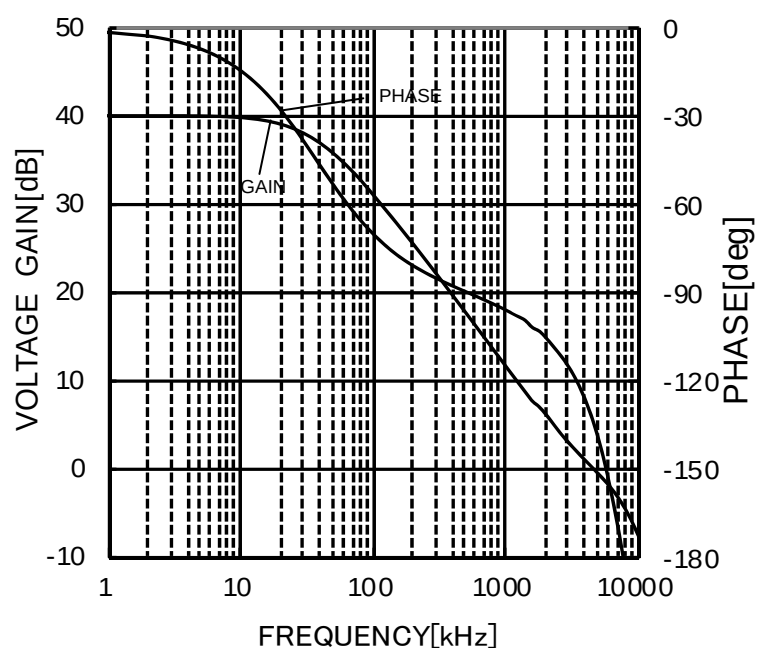
Figure 45. Voltage Gain • Phase - Frequency ( V_{CC}/V_{EE}=+15V/-15V , A_v=40dB , R_L=2k\Omega , C_L=100pF , T_a=25^\circ C )
