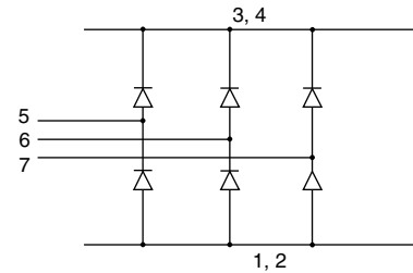
Electrical circuit
