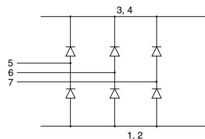
Electrical circuit
