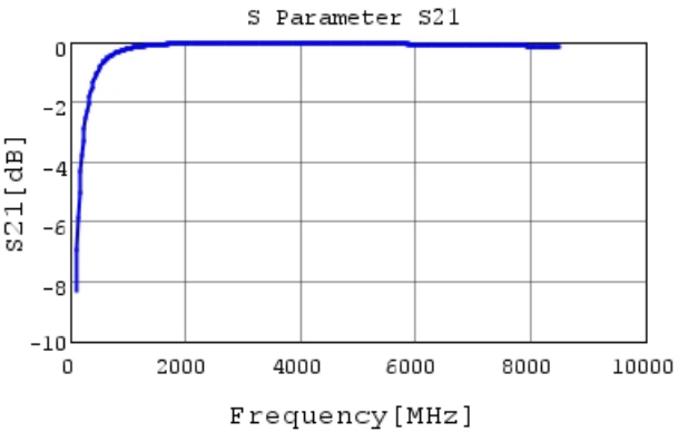
GCQ1555C1H6R6WB01 S21 DCOV, 25degC
