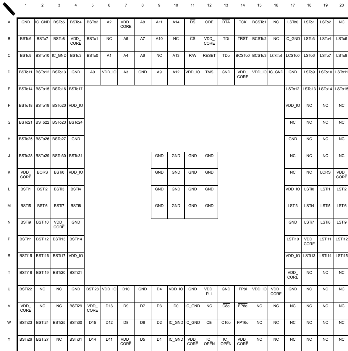
Figure 2 - ZL50057 PBGA Connections (272 PBGA, 27 mm x 27 mm) Pin Diagram (as viewed through top of package)
