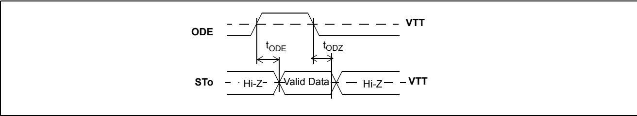
Figure 34 - Output Driver Enable (ODE)
