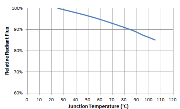
Fig.4 Relative Radiant Flux vs. Junction Temperature
