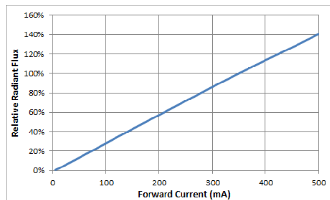
Fig.2 Relative Radiant Flux vs. Forward Current
