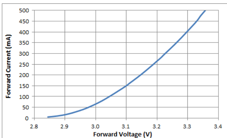
Fig. 3 Forward Current vs. Forward Voltage
