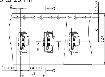
SECT. G-G
