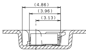
SECT. F-F
