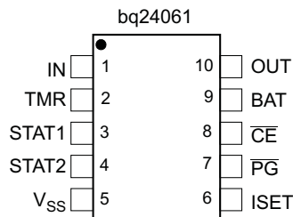
Pin Out (Top View)
