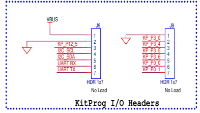
I2C & UART Connection
