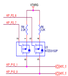
I2C & UART Connection
