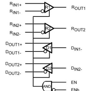
Figure 2. Functional Diagram
