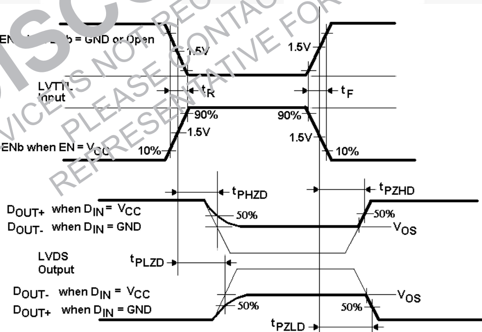
Figure 8. LVDS Output Enable / Disable Timing Waveforms
