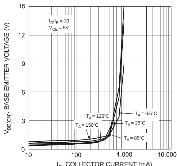
Fig. 8 V_{BE(ON)} vs. I_C @ V_{CE} = 5V
