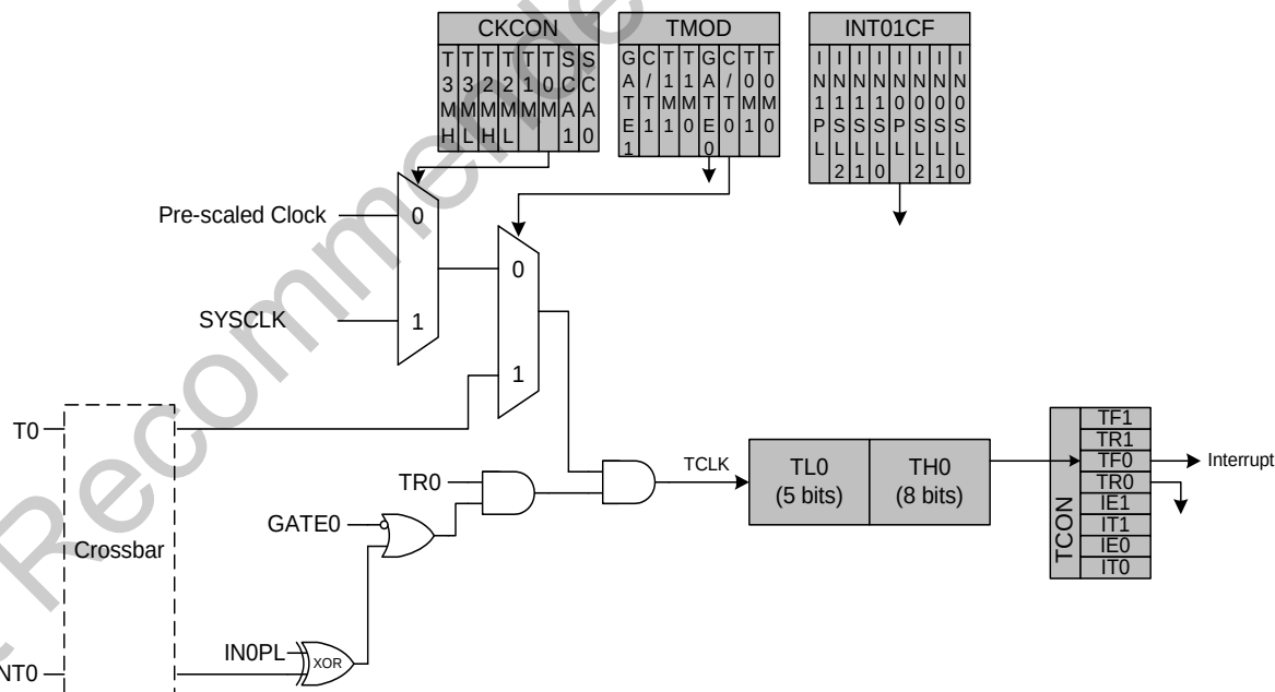
Figure 19.1. T0 Mode 0 Block Diagram
