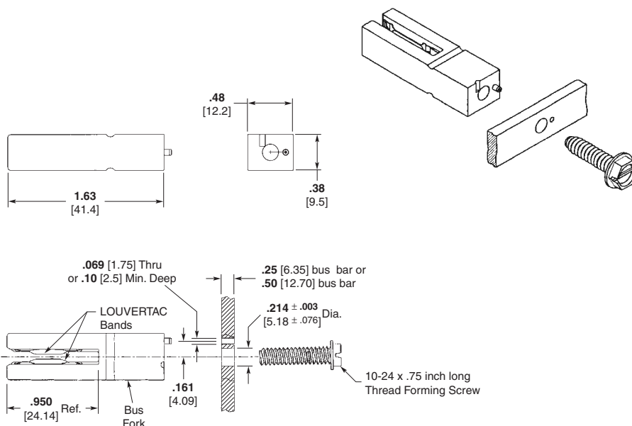
Part Number 194257-1
