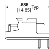
Part Number 5787142-1
