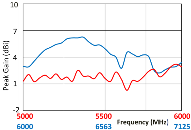
Peak Gain
