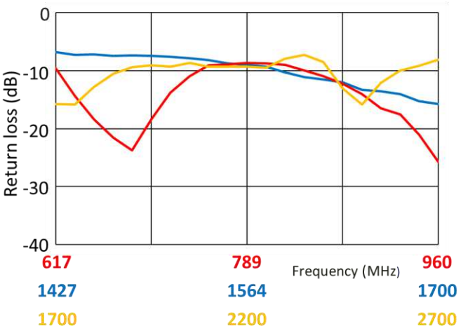
Return Loss
