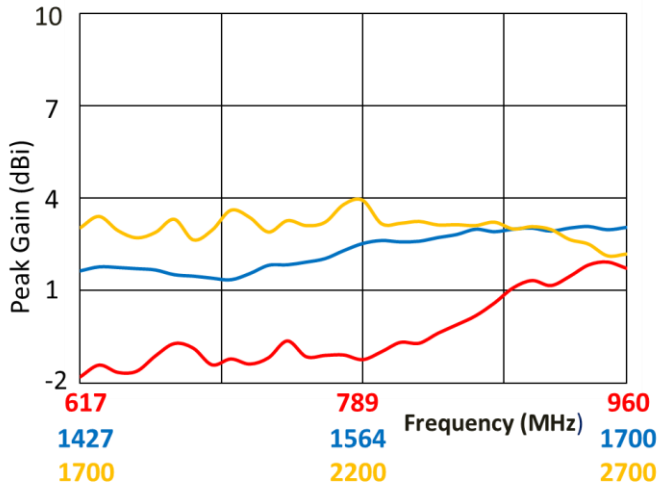
Peak Gain
