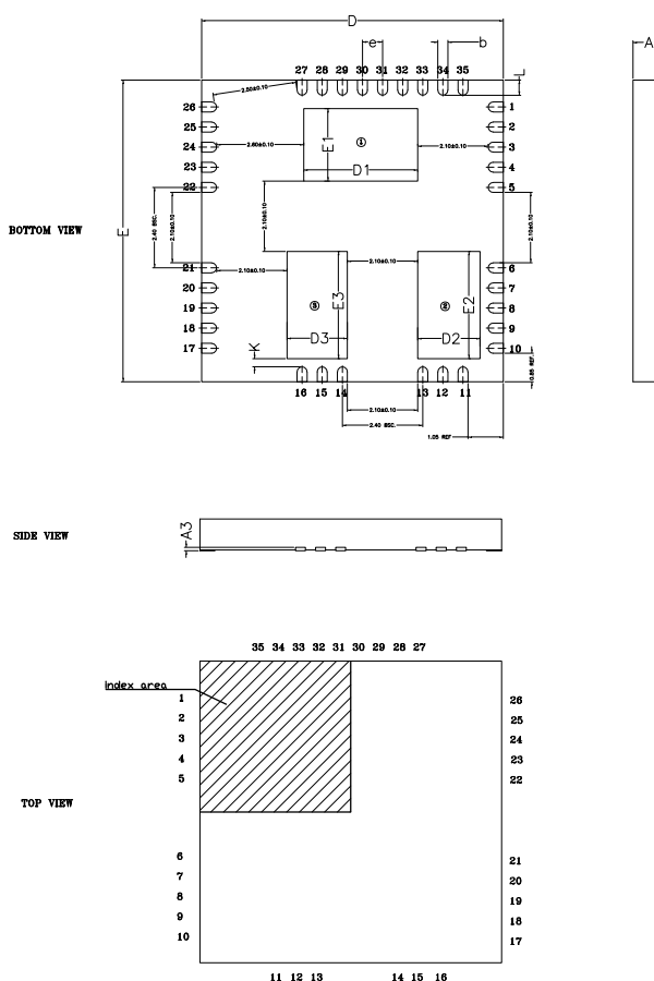
Figure 41. Package outline
