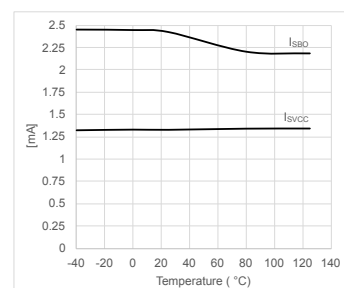
Figure 26. Switching current consumption vs. TJ (ISCC, ISBO)
