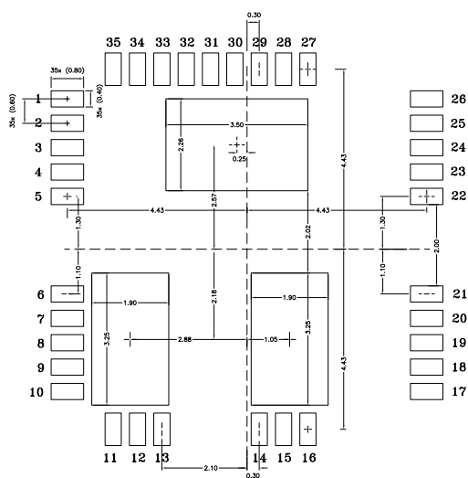
Figure 42. Suggested footprint
