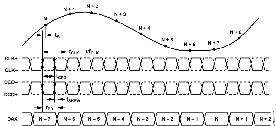
Figure 2. Single Port Mode
