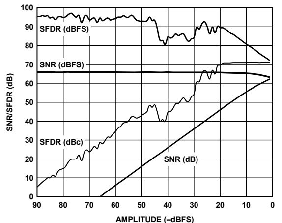
Figure 16. AD9626-170 SNR/SFDR vs. Input Amplitude; 140.3 MHz
