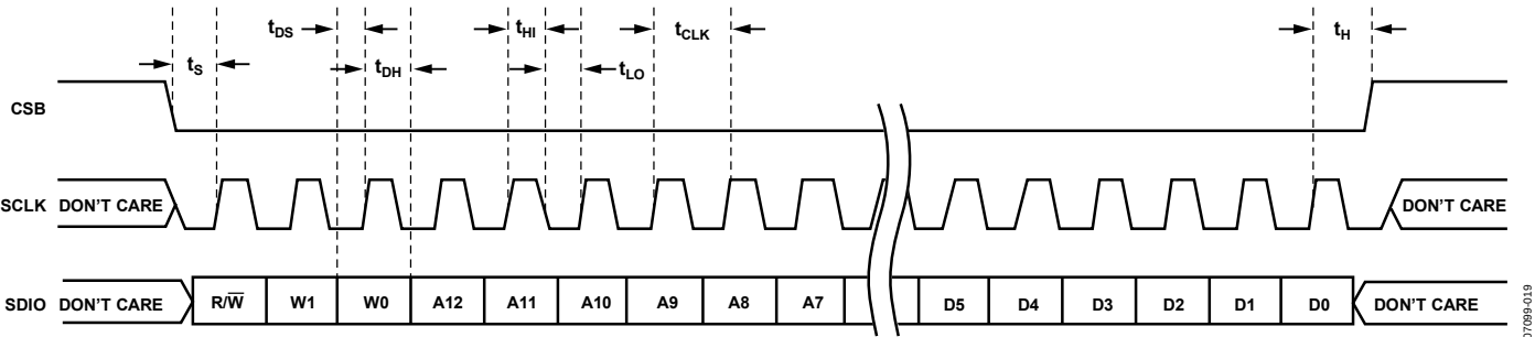
Figure 53. Serial Port Interface Timing Diagram
