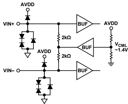
Figure 6. Analog Inputs ( V_{CML} = \sim 1.4\text{ V} )
