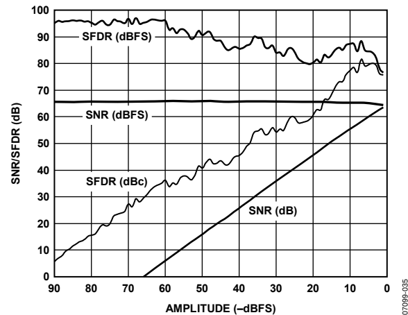
Figure 26. AD9626-210 SNR/SFDR vs. Input Amplitude; 210 MSPS, 170.3 MHz
