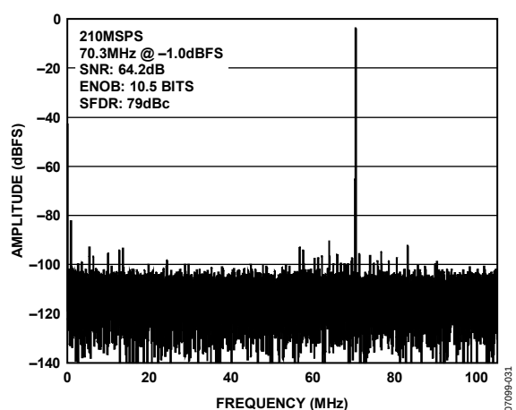
Figure 22. AD9626-210 64k Point Single-Tone FFT; 210 MSPS, 70.3 MHz
