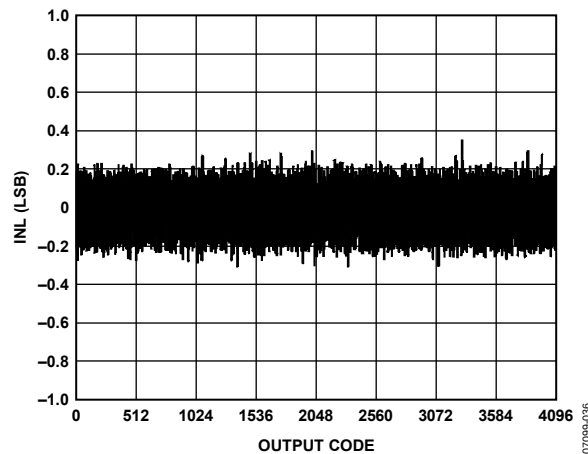
Figure 27. AD9626-210 INL; 210 MSPS
