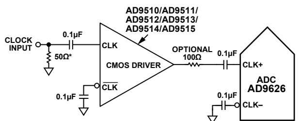
Figure 49. Single-Ended 3.3 V CMOS Sample Clock
