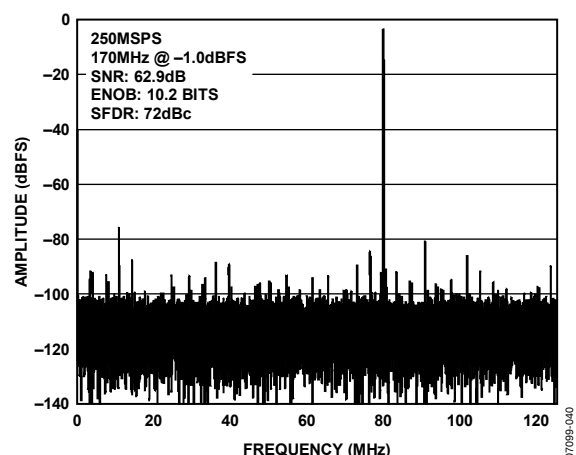
Figure 32. AD9626-250 64k Point Single-Tone FFT; 250 MSPS, 170.3 MHz
