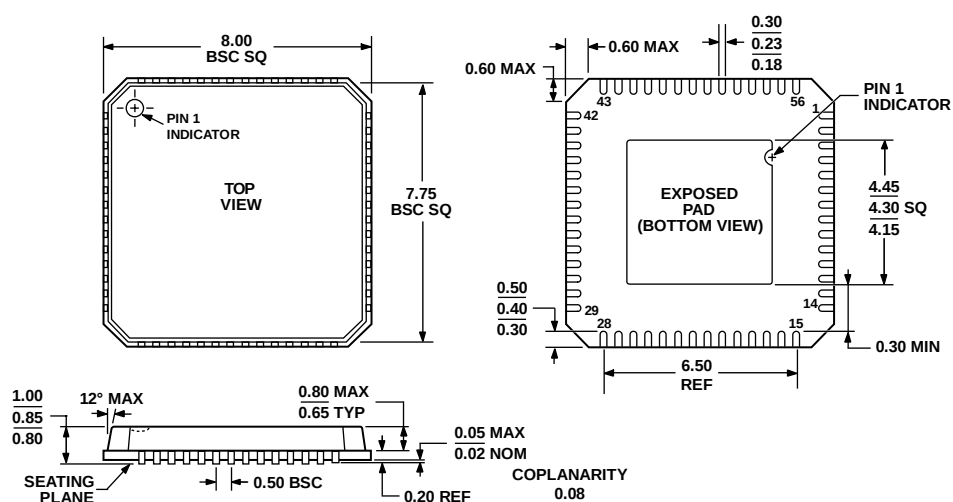
COMPLIANT TO JEDEC STANDARDS MO-220-VLLD-2 Figure 58. 56-Lead Lead Frame Chip Scale Package [LFCSP_VQ] 8 mm x 8 mm Body, Very Thin Quad (CP-56-2) Dimensions shown in millimeters
