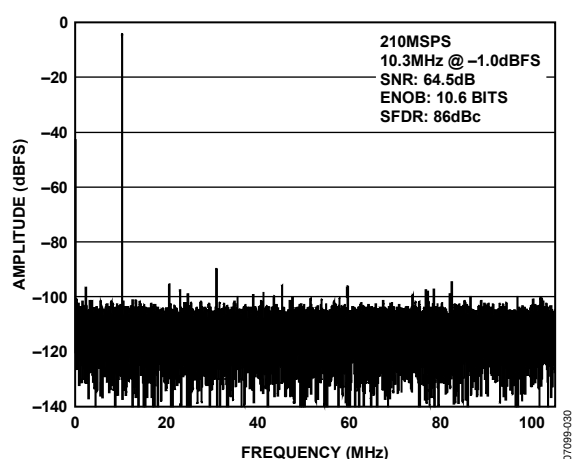
Figure 21. AD9626-210 64k Point Single-Tone FFT; 210 MSPS, 10.3 MHz
