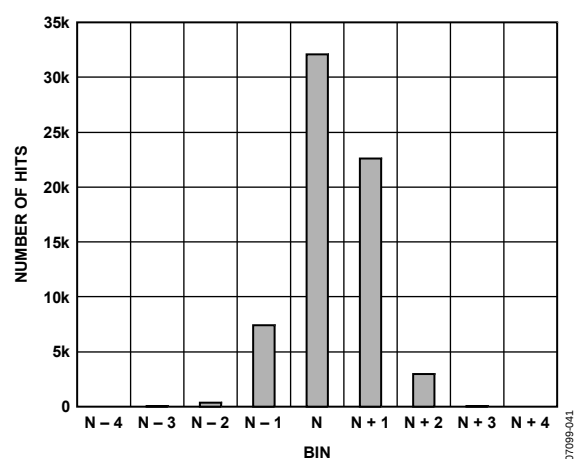
Figure 33. AD9626-250 Grounded Input Histogram; 250 MSPS
