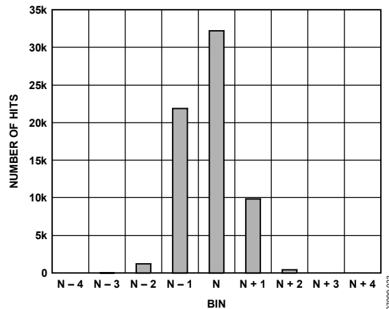
Figure 14. AD9626-170 Grounded Input Histogram; 170 MSPS
