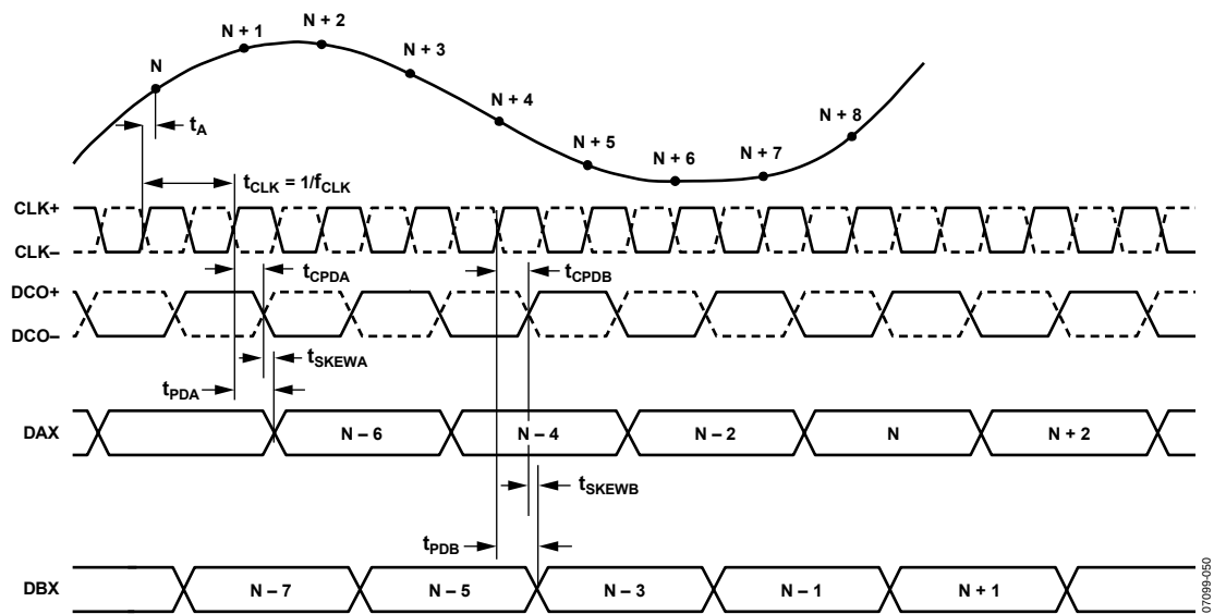
Figure 3. Interleaved Mode
