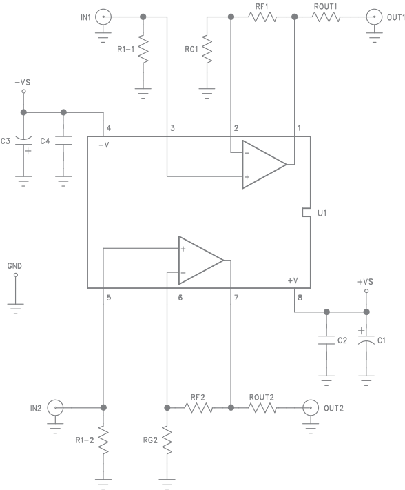
Figure 9. CEB006 Schematic
