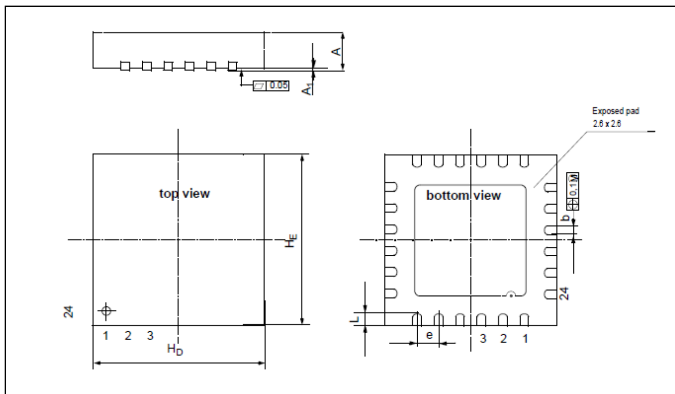
Figure 10: 24-pin QFN Package Drawing
