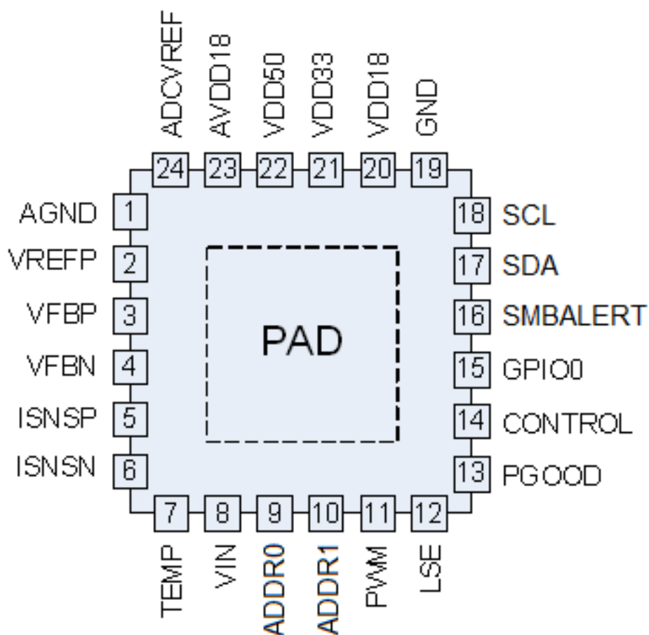
Figure 2: Pin Out Diagram (Top View)
