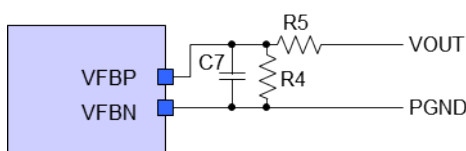
Figure 7: Output Voltage Sense Circuitry
