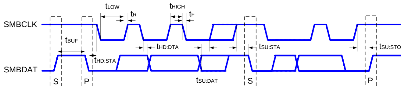
Figure 6: PMBus™ Timing Diagram
