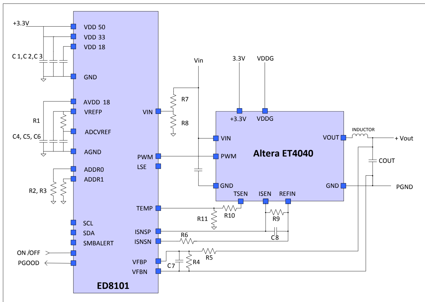
Figure 9: Application Circuit with a 3.3V Supply Voltage
