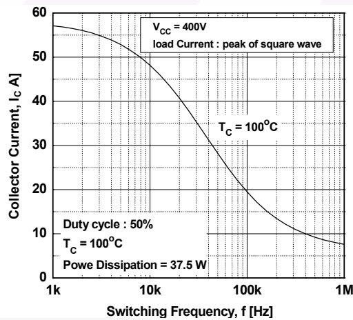
Figure 21. Load Current Vs. Frequency
