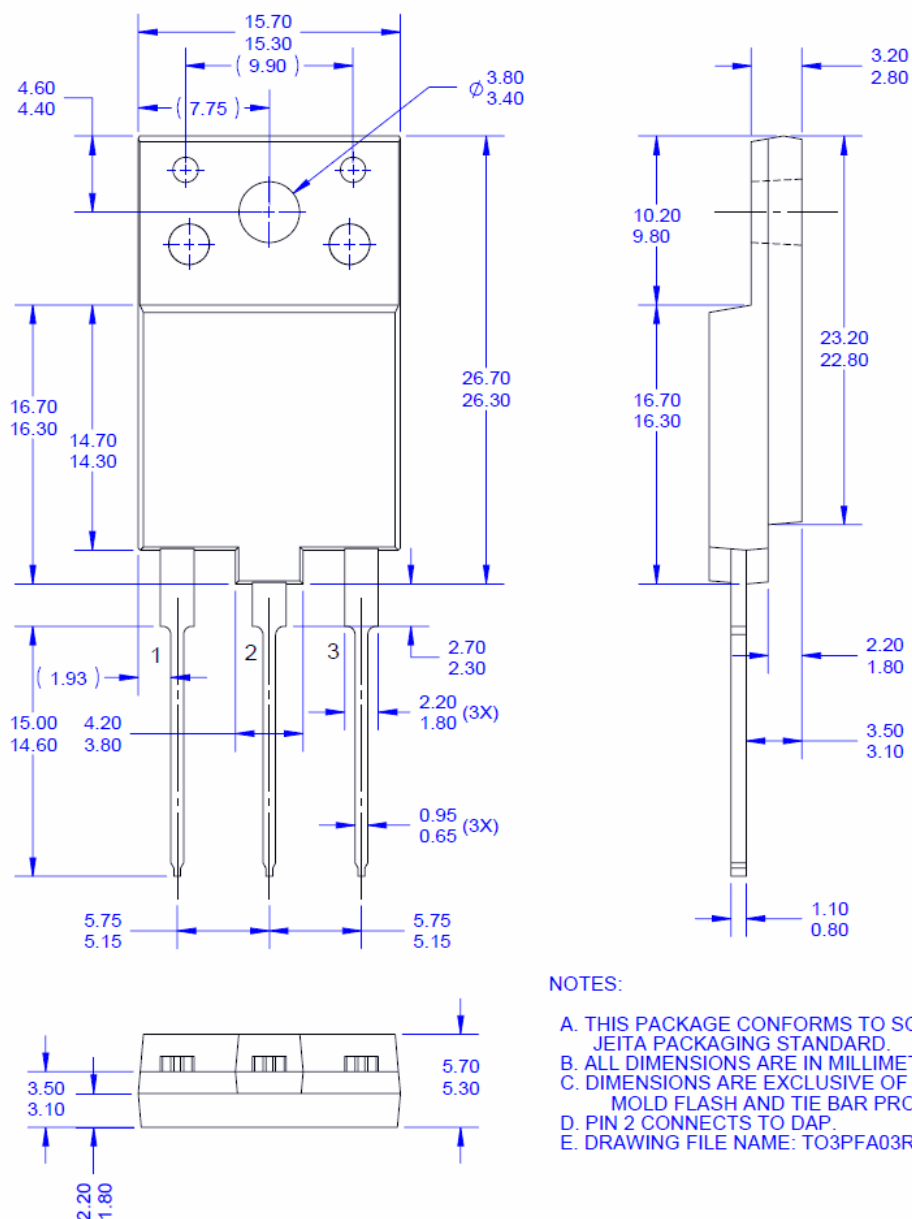
Figure 28. TO3PF,MOLDED,3LD,FULLPACK (AG)
