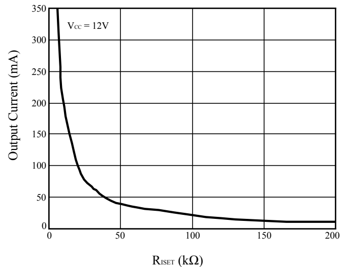
Figure 10 Output Current vs. R_{ISET}
