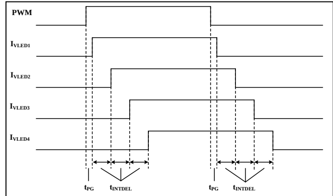
Figure 15 PWM Dimming Sequential On/Off
