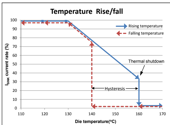
Figure 18 Temperature regulation
