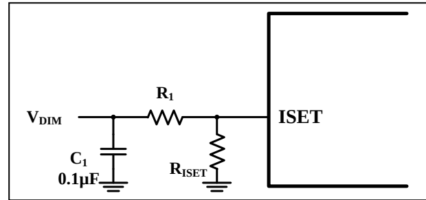
Figure 16 Analog Dimming
