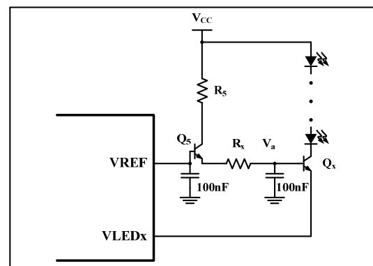
Figure 17 IS31LT3117 with external BJTs
