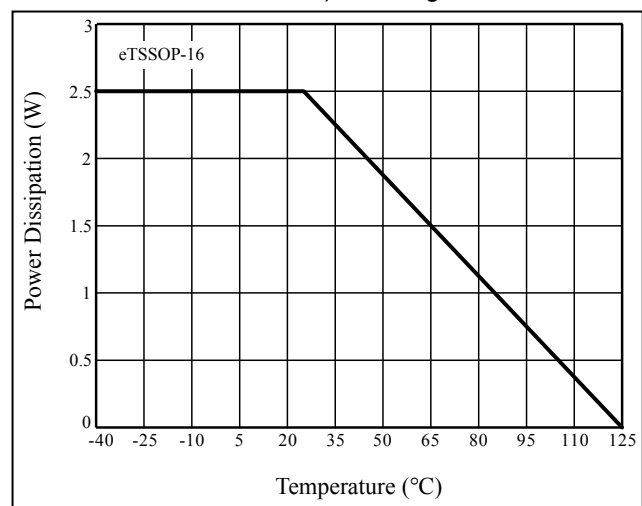
Figure 19 Dissipation Curve
