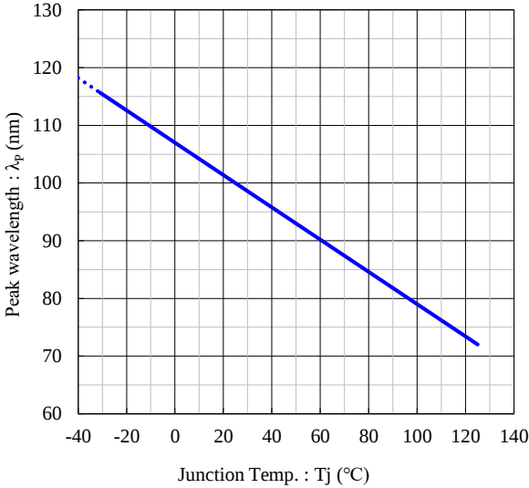
Junction temp. vs. Peak wavelength
