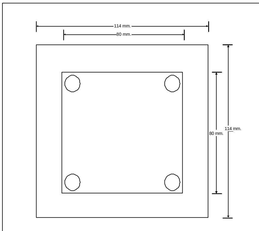
Figure 4. Bottom View
