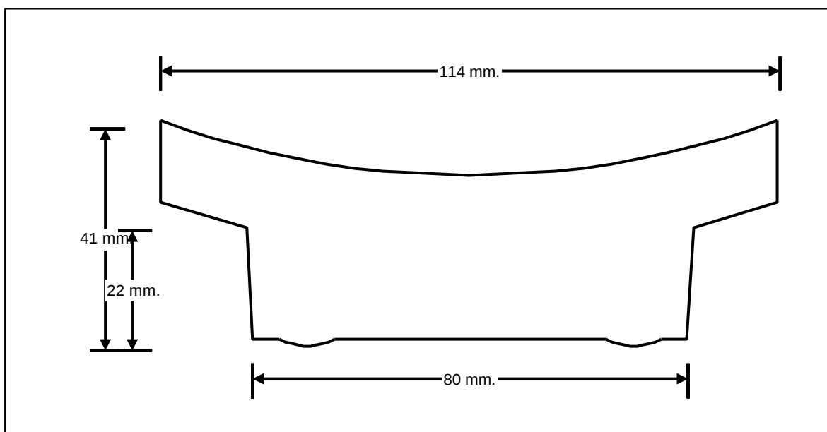
Figure 3. Side View
