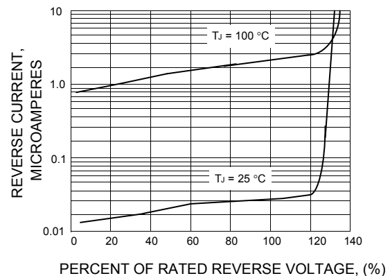
FIG.5 - TYPICAL REVERSE CHARACTERISTICS PER DIODE
