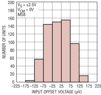
V OS Distribution
