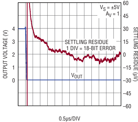
18-Bit Settling Time to 4V p-p Output Step
