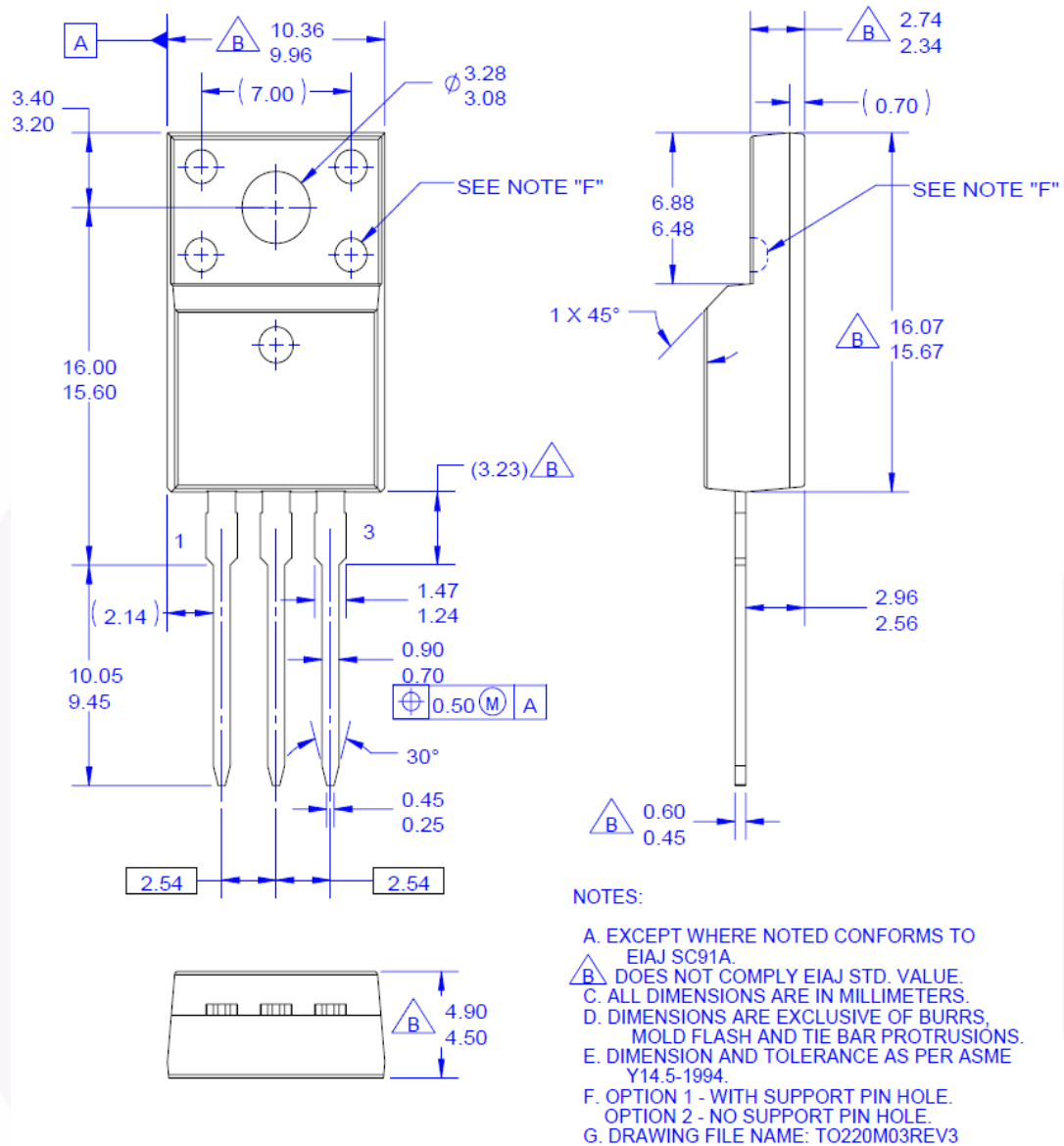
Figure 23. TO-220F 3L - TO220, MOLDED, 3LD, FULL PACK, EIAJ SC91, STRAIGHT LEAD
