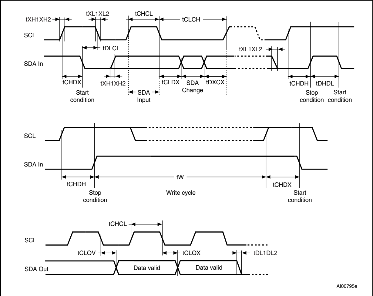
Figure 13. AC waveforms
