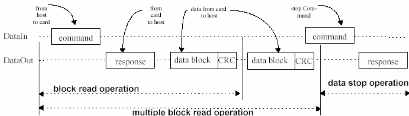
Figure 11: Read operation
