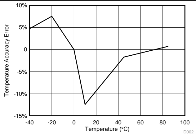
Figure 13. Internal Temperature Accuracy Error
