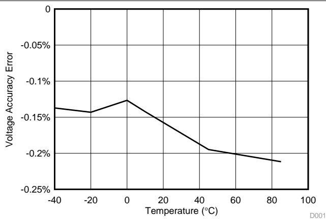
Figure 12. Voltage Accuracy Error
