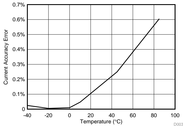
Figure 14. Current Accuracy Error
