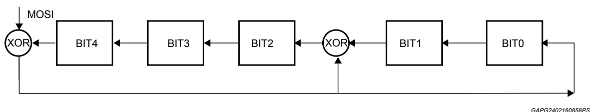
Figure 23. Structure of CRC generator
