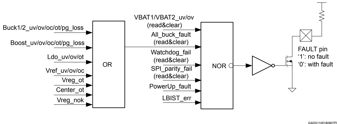
Figure 13. Fault function in active mode
