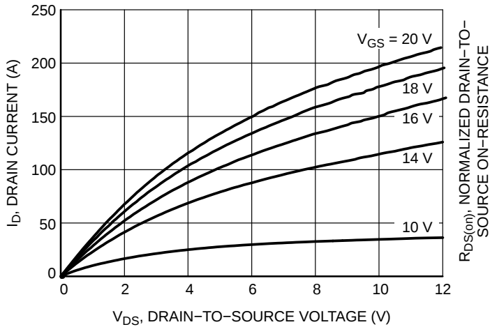
Figure 1. On-Region Characteristics
