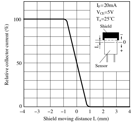
Fig.14 Relative Collector Current vs. Shield Distance (2)
