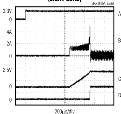
STARTUP WAVEFORM (LIGHT LOAD)
