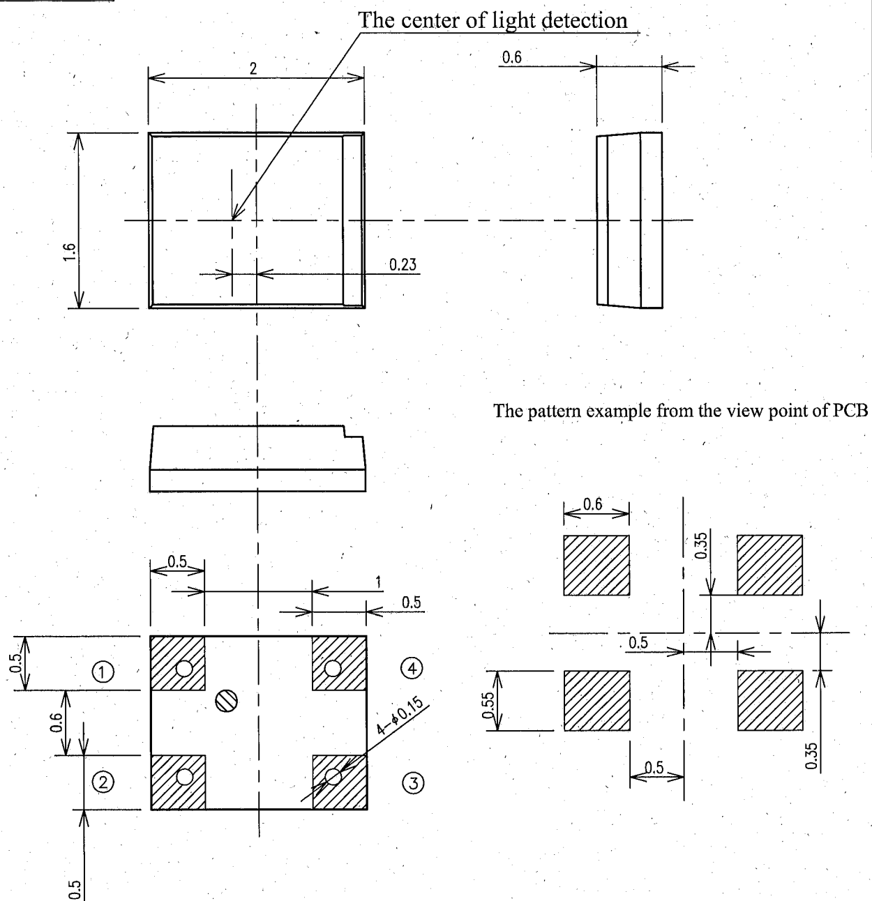
Pin arrangement
