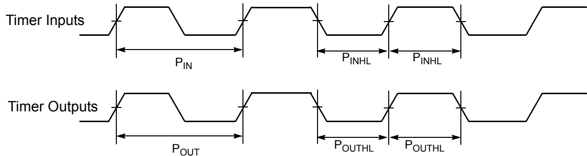
Figure 10-15 Timer Timing
